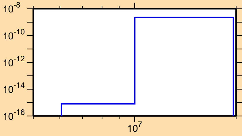
\sigma vs. E for ^{166}\text{W}(\text{mt117})
