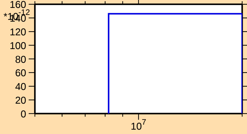
\sigma vs. E for ^{166}\text{W}(\text{n},\text{pt})
