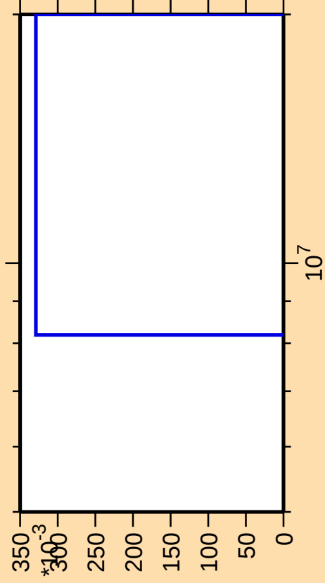
\Delta\sigma/\sigma vs. E for ^{166}\text{W}(n,nt)
