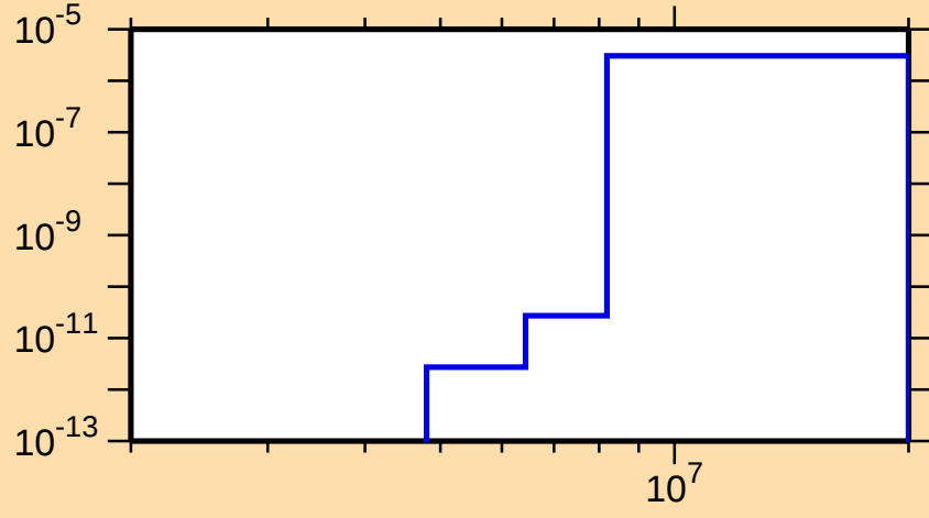
\sigma vs. E for ^{166}\text{W}(n,\text{He3})
