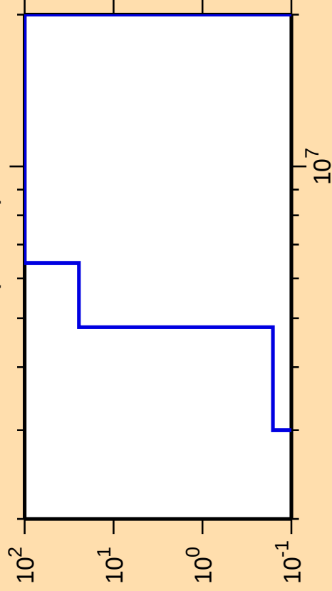
\Delta\sigma/\sigma vs. E for ^{166}\text{W}(n,\text{He3})
