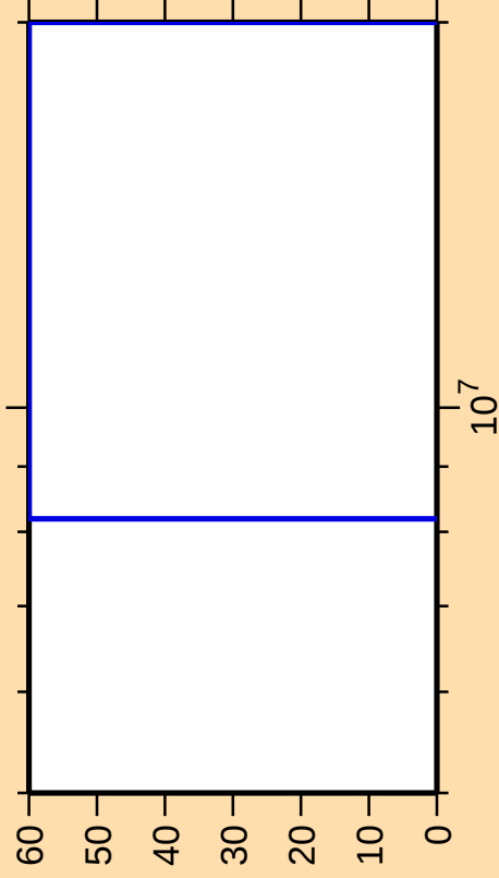
\Delta\sigma/\sigma vs. E for ^{166}\text{W}(\text{n},\text{pt})
