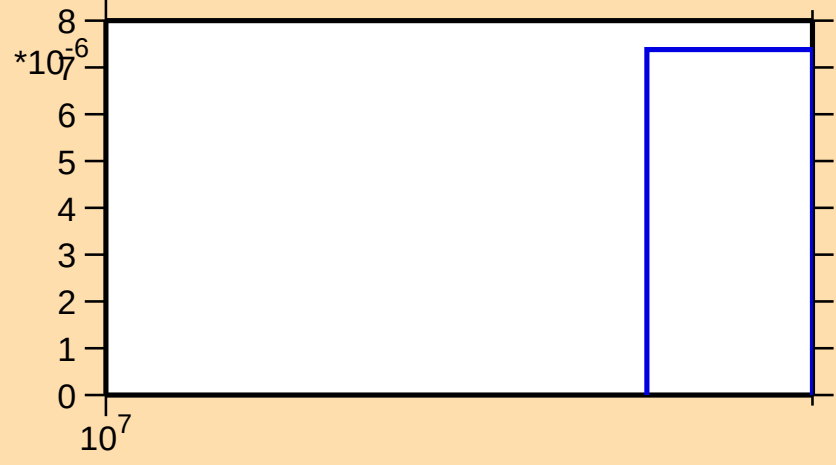
\sigma vs. E for ^{168}\text{W}(n,3n)
