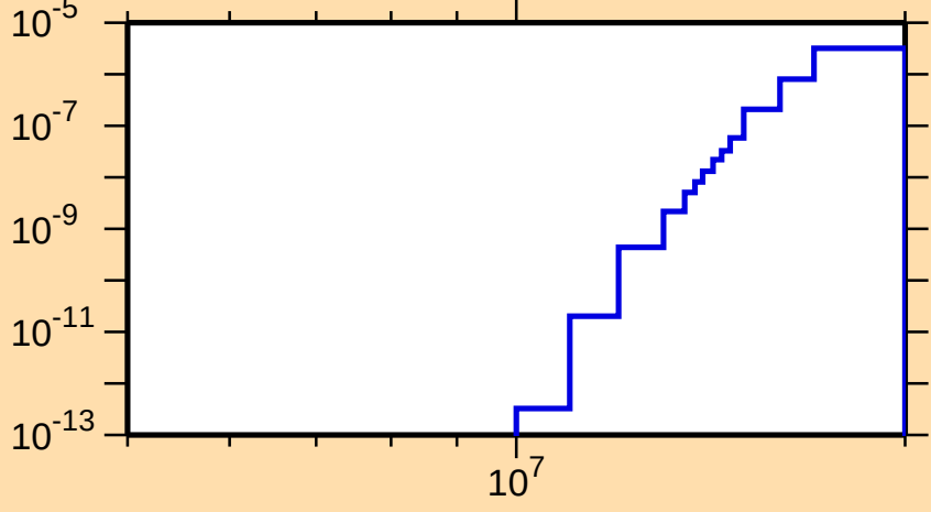
\sigma vs. E for ^{168}\text{W}(n,\text{pd})
