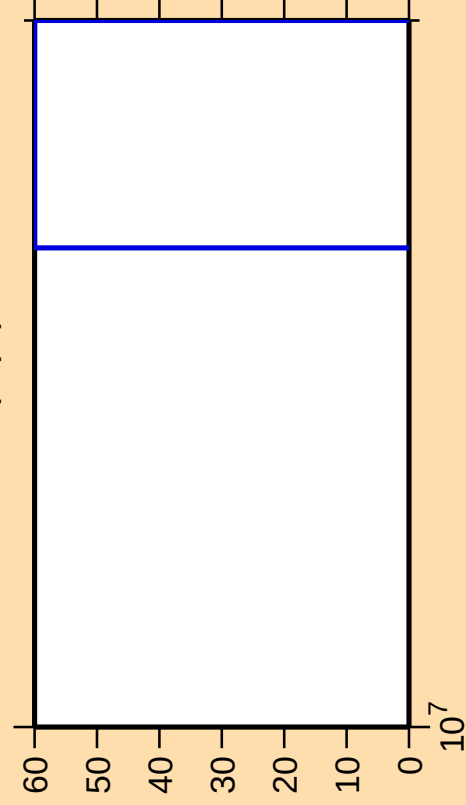
\Delta\sigma/\sigma vs. E for ^{168}\text{W}(\text{n},\text{pt})
