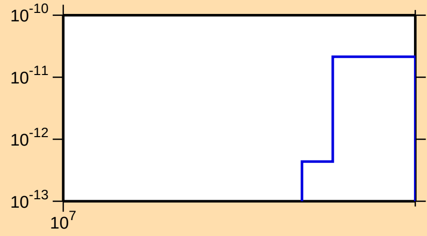
\sigma vs. E for ^{168}\text{W} (mt 34)
