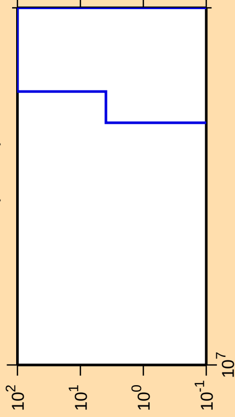
\Delta\sigma/\sigma vs. E for ^{168}\text{W} (mt 34)
