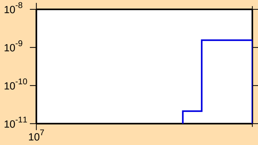
\sigma vs. E for ^{168}\text{W}(\text{n},\text{pt})
