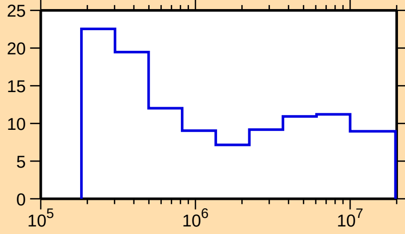
\Delta\sigma/\sigma vs. E for ^{168}\text{W}(\text{n,tot.})
