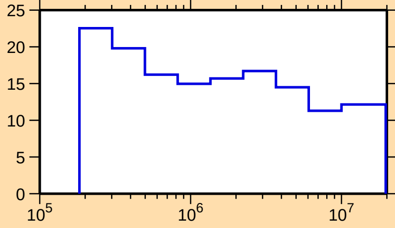
\Delta\sigma/\sigma vs. E for ^{168}\text{W}(\text{n,el.})
