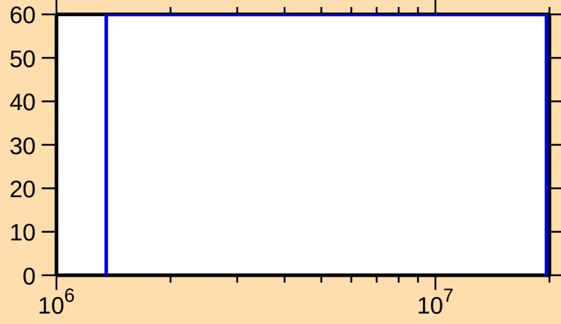
\Delta\sigma/\sigma vs. E for ^{168}\text{W}(n,n_1)
