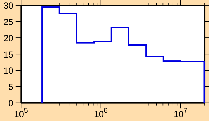
\Delta\sigma/\sigma vs. E for ^{168}\text{W}(\text{n,nonel.})
