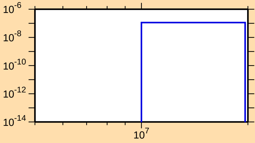
\sigma vs. E for ^{168}\text{W}(n,\text{pd})
