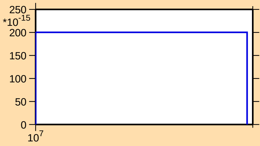
\sigma vs. E for ^{168}\text{W} (mt 34)
