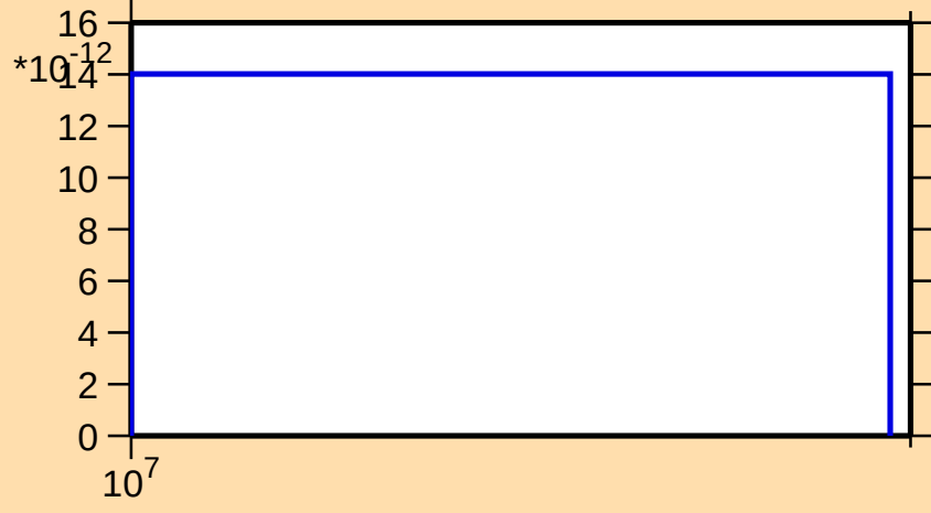
\sigma vs. E for ^{168}\text{W}(\text{n},\text{pt})
