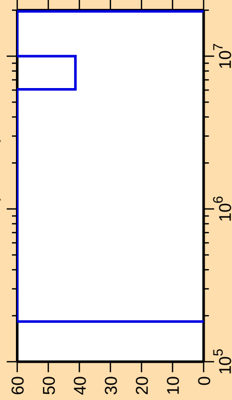
\Delta\sigma/\sigma vs. E for ^{168}\text{W}(\text{n,inel.})
