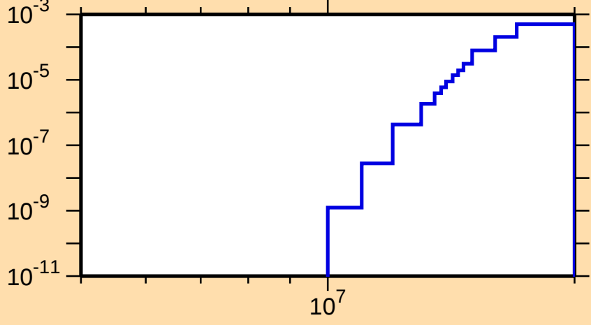
\sigma vs. E for ^{169}\text{W}(n,2n\alpha)
