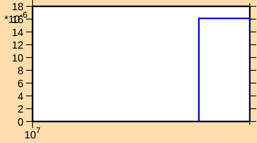
\sigma vs. E for ^{169}\text{W}(n,3n)
