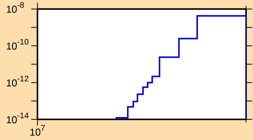
\sigma vs. E for ^{169}\text{W} (mt 34)
