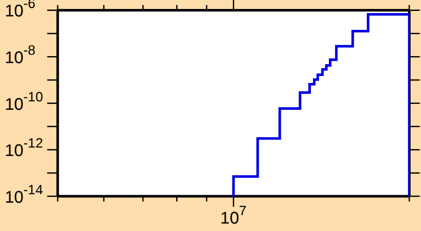
\sigma vs. E for ^{169}\text{W}(\text{mt 45})
