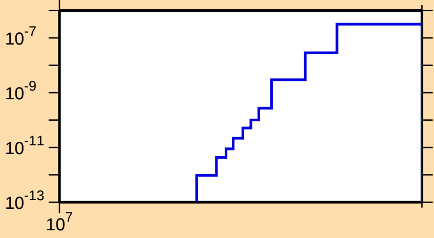
\sigma vs. E for ^{169}\text{W}(n,\text{pt})
