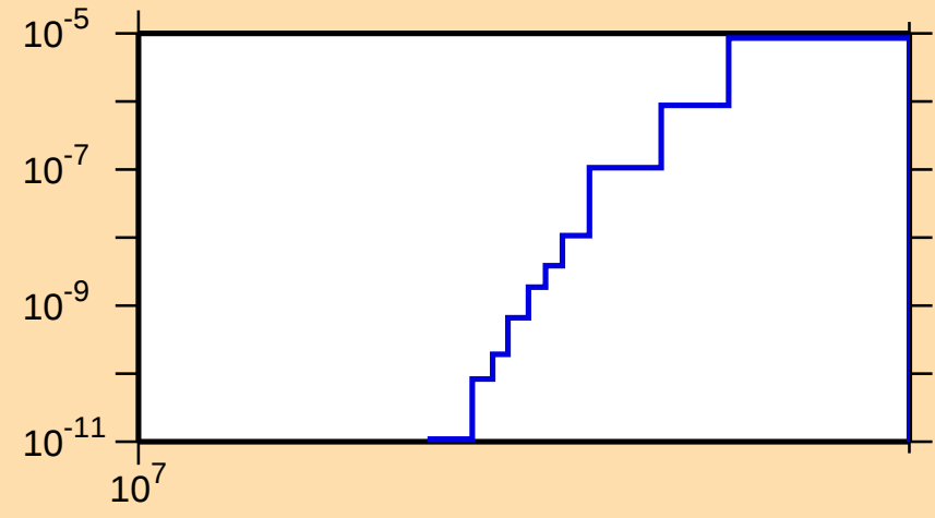
\sigma vs. E for ^{169}\text{W}(n,\text{nd})
