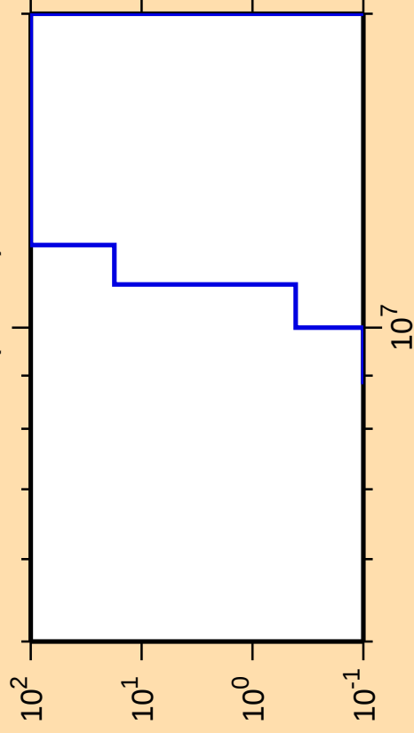
\Delta\sigma/\sigma vs. E for ^{169}\text{W}(\text{mt 45})
