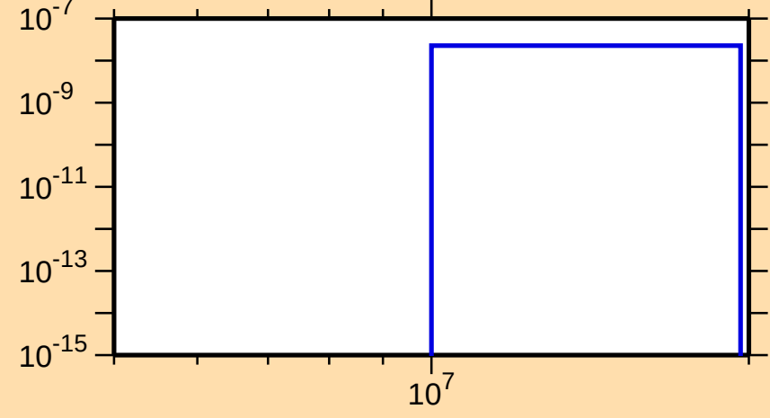
\sigma vs. E for ^{169}\text{W}(n,\text{pd})
