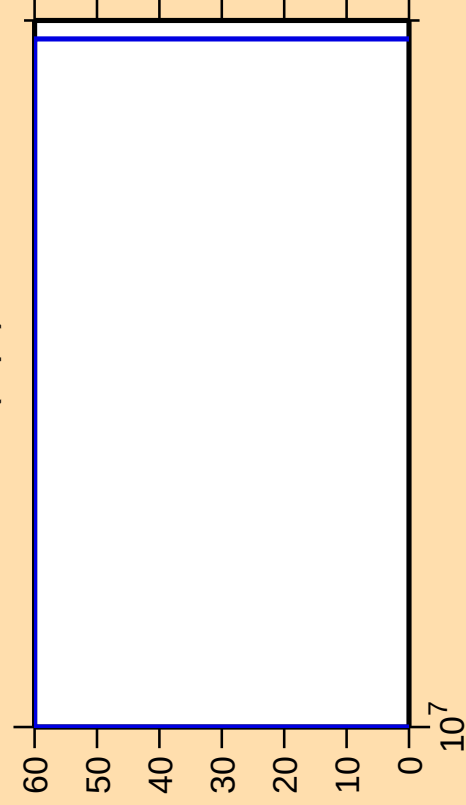
\Delta\sigma/\sigma vs. E for ^{169}\text{W}(\text{n},\text{pt})
