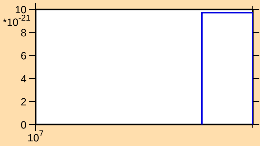
\sigma vs. E for ^{178}\text{W} (mt 11)
