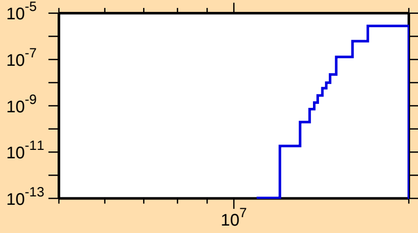
\sigma vs. E for ^{178}\text{W}(n,2n\alpha)
