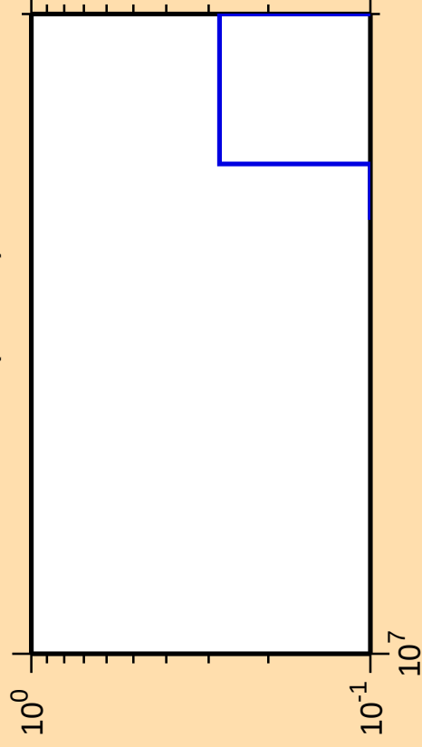
\Delta\sigma/\sigma vs. E for ^{178}\text{W}(n,3n\alpha)
