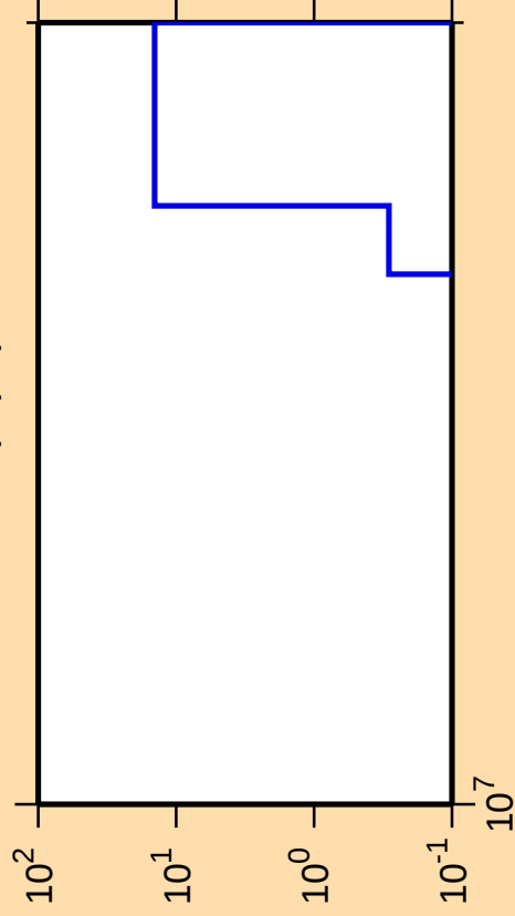
\Delta\sigma/\sigma vs. E for ^{178}\text{W}(\text{n},\text{pd})
