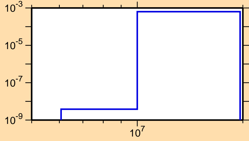
\sigma vs. E for ^{178}\text{W}(n,d)
