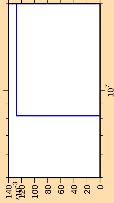
\Delta\sigma/\sigma vs. E for ^{178}\text{W}(n,\text{pd})
