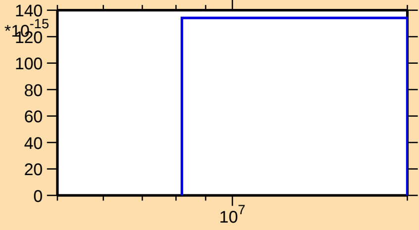
\sigma vs. E for ^{178}\text{W}(\text{mt } 45)
