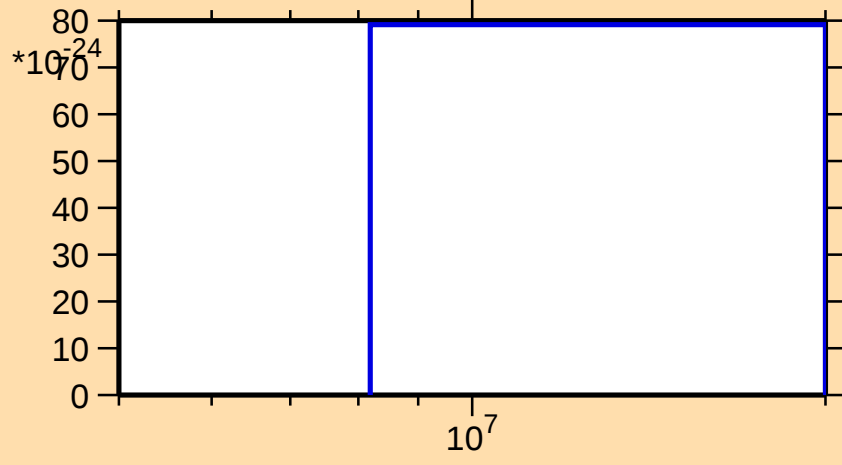
\sigma vs. E for ^{178}\text{W}(\text{mt 11})
