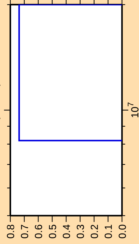
\Delta\sigma/\sigma vs. E for ^{178}\text{W}(\text{mt } 45)
