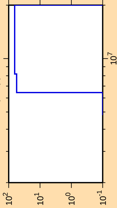
\Delta\sigma/\sigma vs. E for ^{178}\text{W}(n,np)
