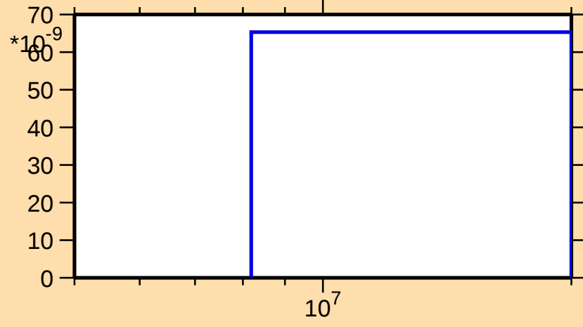
\sigma vs. E for ^{178}\text{W}(n,2n\alpha)
