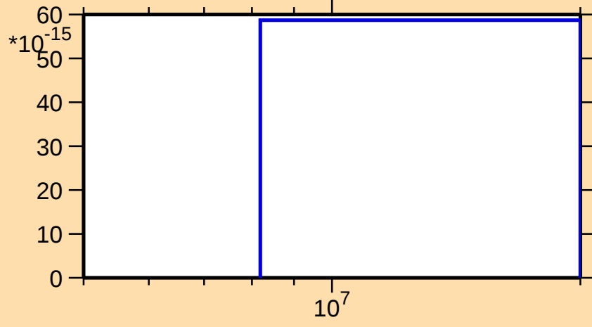
\sigma vs. E for ^{178}\text{W}(\text{mt117})
