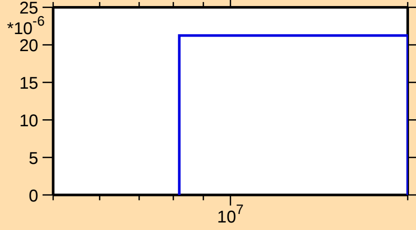
\sigma vs. E for ^{178}\text{W}(n,t)
