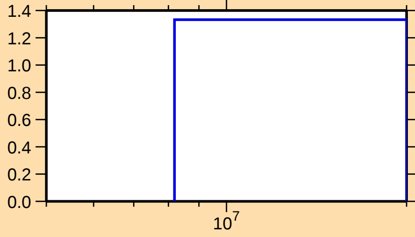
\sigma vs. E for ^{178}\text{W}(n,2n)
