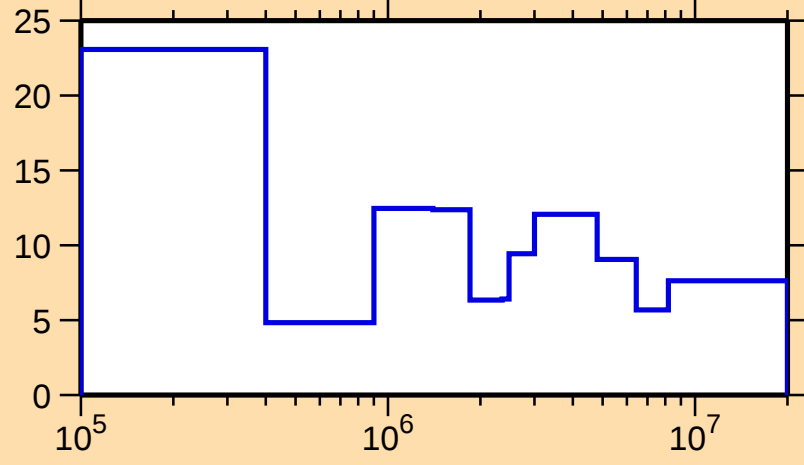
\Delta\sigma/\sigma vs. E for ^{178}\text{W}(\text{n,el.})
