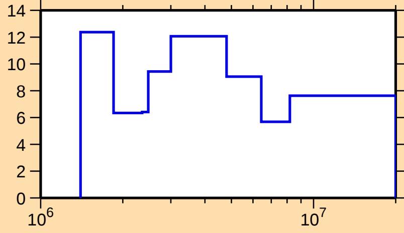
\Delta\sigma/\sigma vs. E for ^{178}\text{W}(\text{n},\text{el.})
