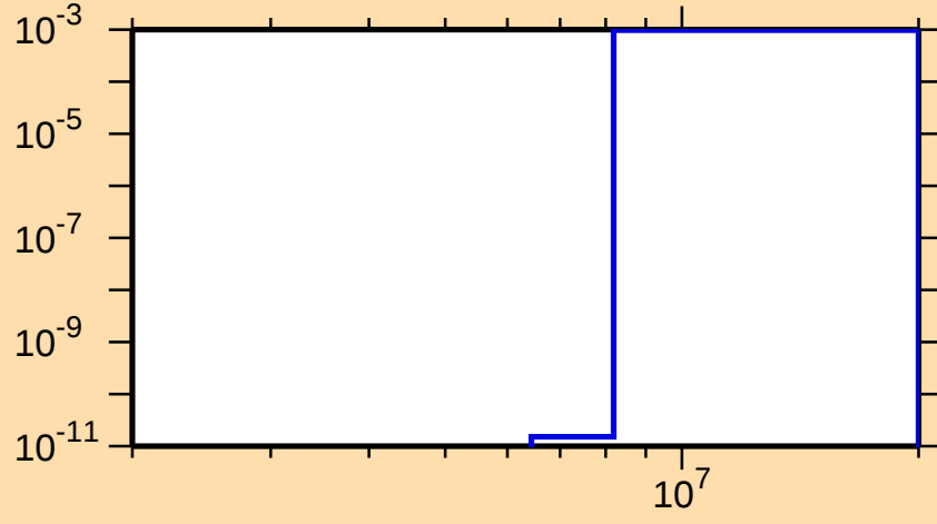
\sigma vs. E for ^{178}\text{W}(n,np)
