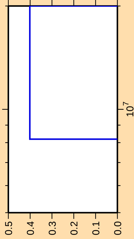
\Delta\sigma/\sigma vs. E for ^{178}\text{W}(\text{mt117})
