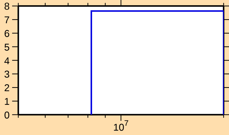
\Delta\sigma/\sigma vs. E for ^{178}\text{W}(n,\text{el.})
