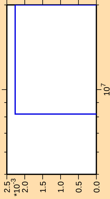
\Delta\sigma/\sigma vs. E for ^{178}\text{W}(n,3n\alpha)
