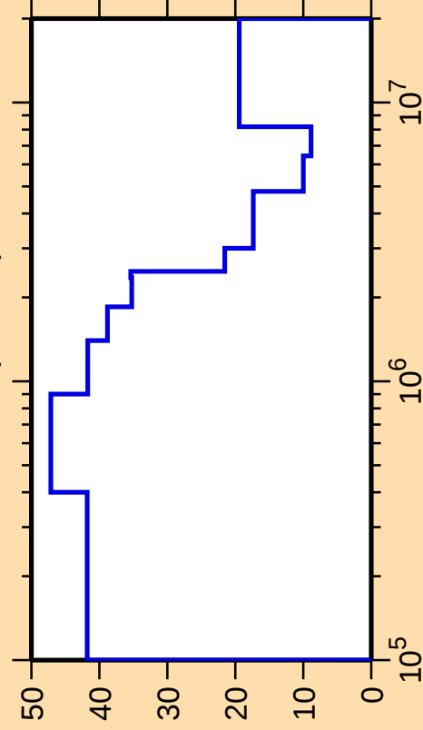
\Delta\sigma/\sigma vs. E for ^{178}\text{W}(\text{n,inel.})
