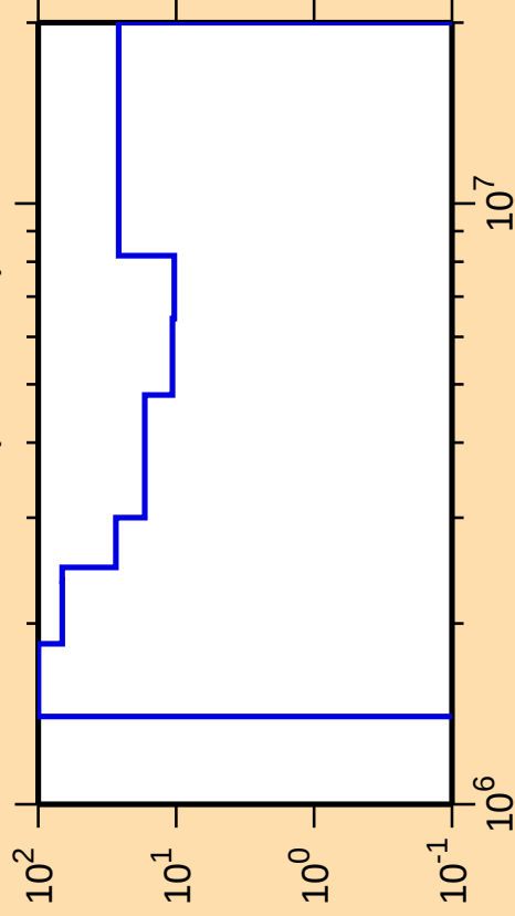
\Delta\sigma/\sigma vs. E for ^{178}\text{W}(\text{n},\text{ncont.})
