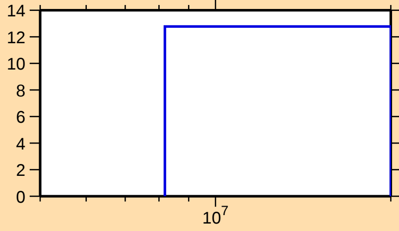
\Delta\sigma/\sigma vs. E for ^{178}\text{W}(n,2n)
