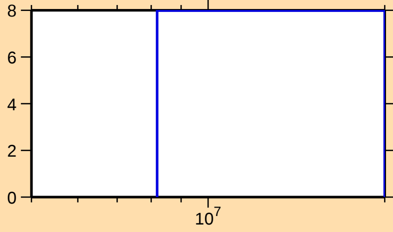
\Delta\sigma/\sigma vs. E for ^{178}\text{W}(n,\text{nonel.})
