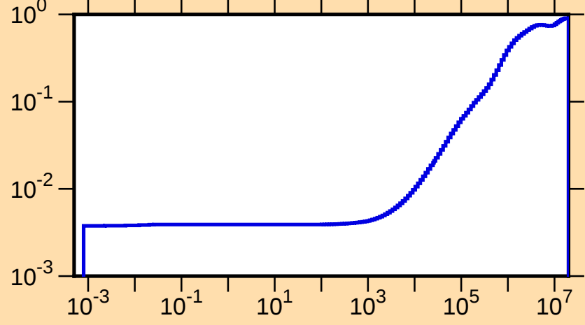
\mu vs. E for ^{179}\text{W}(\text{mt251})
