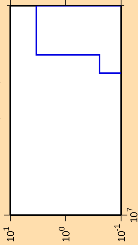
\Delta\sigma/\sigma vs. E for ^{179}\text{W}(\text{mt117})
