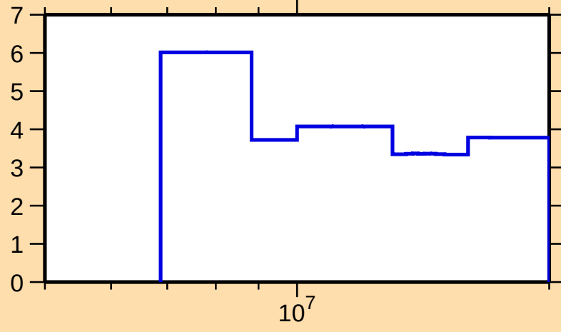
\Delta\sigma/\sigma vs. E for ^{179}\text{W}(n,\text{tot.})
