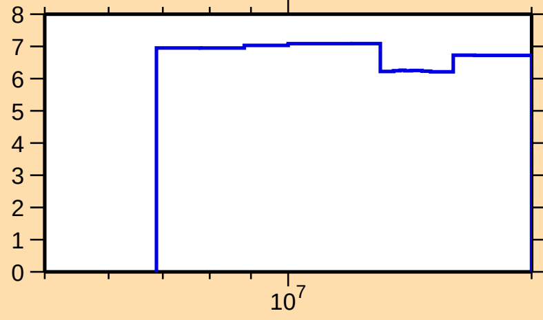
\Delta\sigma/\sigma vs. E for ^{179}\text{W}(n,\text{nonel.})
