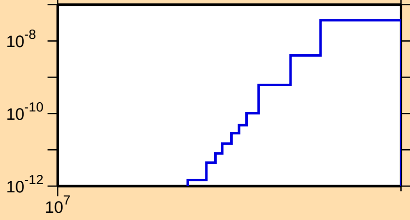
\sigma vs. E for ^{179}\text{W}(n,\text{He3})
