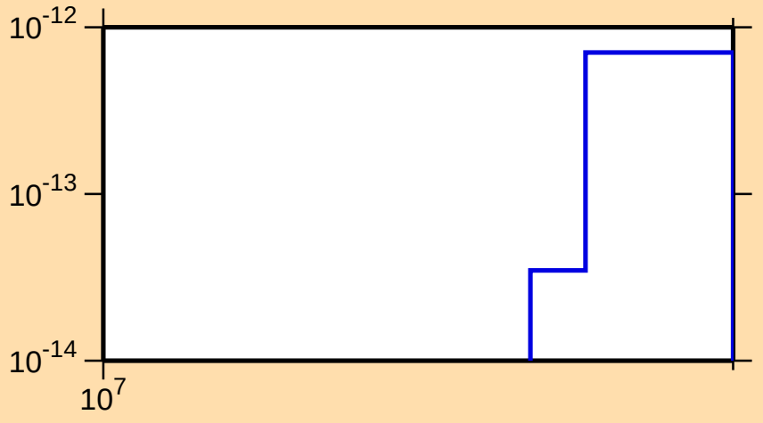
\sigma vs. E for ^{179}\text{W} (mt 45)
