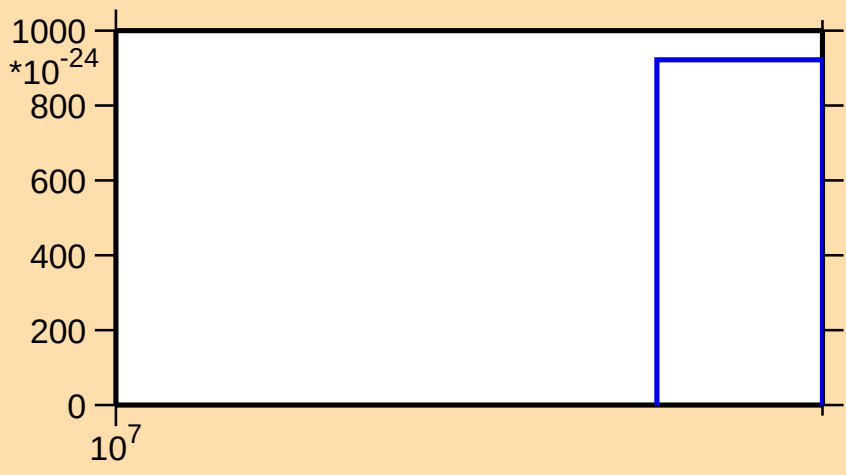
\sigma vs. E for ^{179}\text{W} (mt 11)
