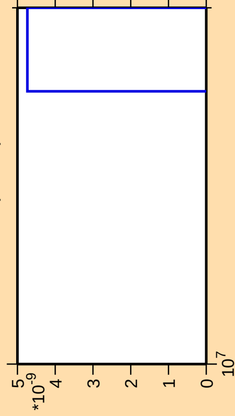
\Delta\sigma/\sigma vs. E for ^{179}\text{W} (mt 11)
