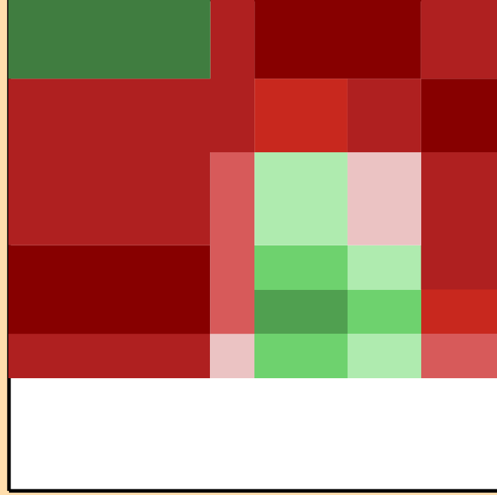
\Delta\sigma/\sigma vs. E for ^{179}\text{W}(n,\text{el.})
