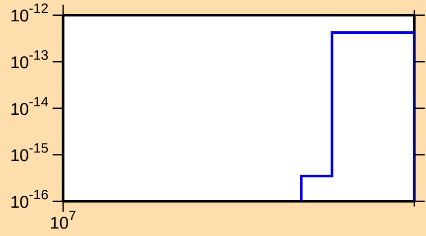
\sigma vs. E for ^{179}\text{W} (mt 34)
