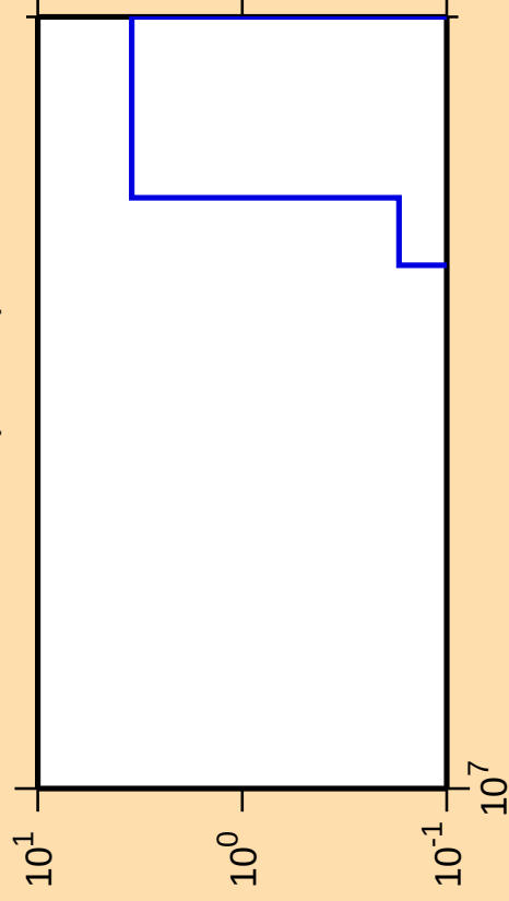
\Delta\sigma/\sigma vs. E for ^{179}\text{W} (mt 45)
