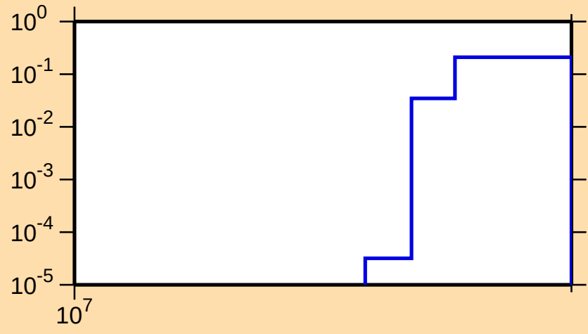
\sigma vs. E for ^{179}\text{W}(n,3n)
