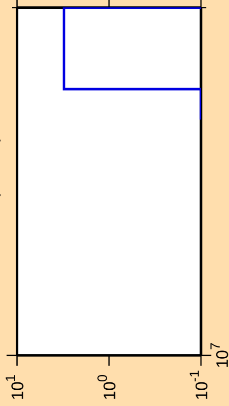
\Delta\sigma/\sigma vs. E for ^{179}\text{W} (mt 34)
