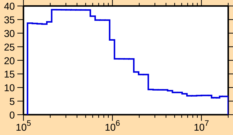
\Delta\sigma/\sigma vs. E for ^{179}\text{W}(\text{n,nonel.})
