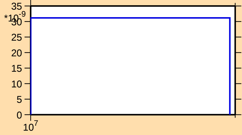
\sigma vs. E for ^{179}\text{W}(\text{n},\text{nd})
