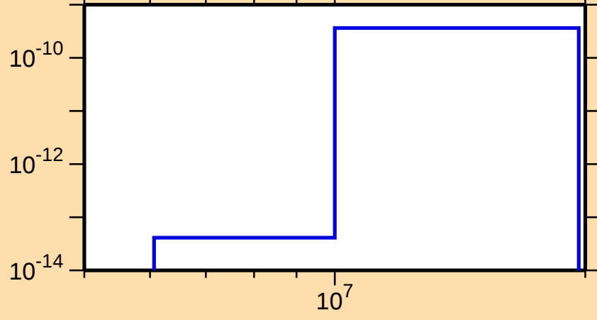
\sigma vs. E for ^{179}\text{W}(n,p\alpha)
