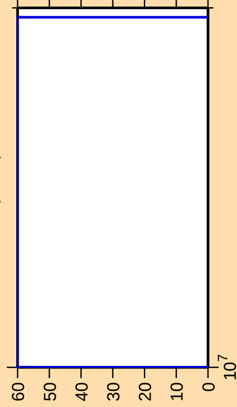
\Delta\sigma/\sigma vs. E for ^{179}\text{W}(\text{n},\text{nd})
