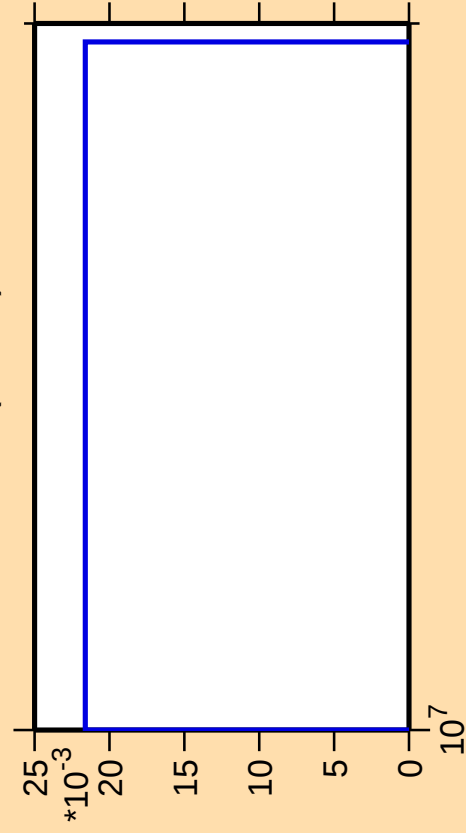
\Delta\sigma/\sigma vs. E for ^{179}\text{W} (mt 34)
