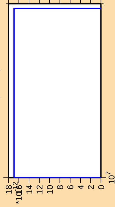
\Delta\sigma/\sigma vs. E for ^{179}\text{W} (mt 11)
