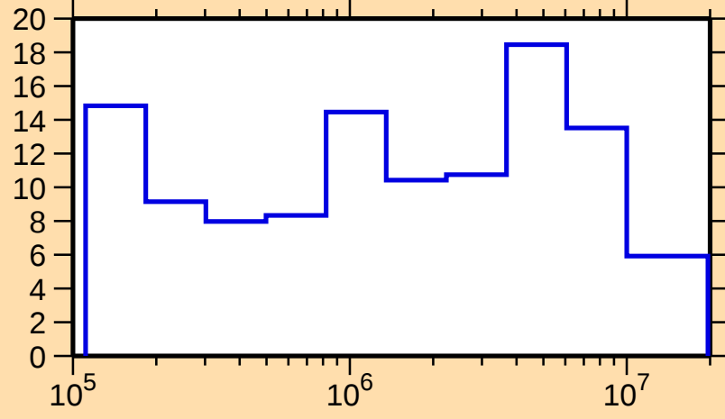
\Delta\sigma/\sigma vs. E for ^{179}\text{W}(\text{n,el.})
