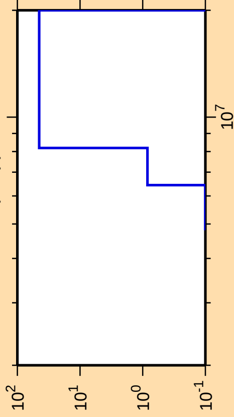
\Delta\sigma/\sigma vs. E for ^{179}\text{W}(n,np)
