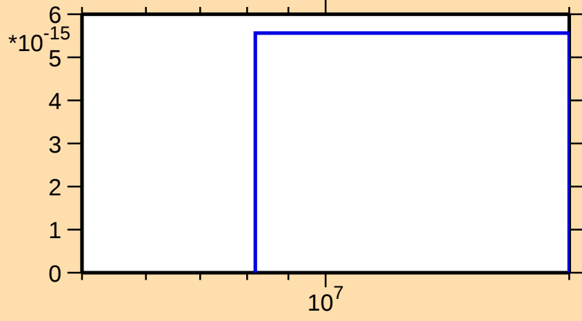
\sigma vs. E for ^{179}\text{W}(\text{mt117})
