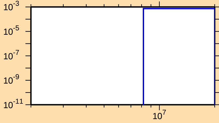
\sigma vs. E for ^{179}\text{W}(n,np)
