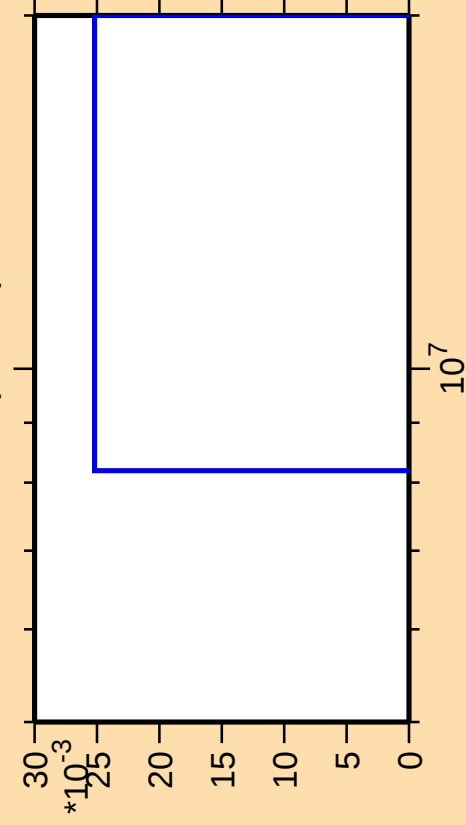
\Delta\sigma/\sigma vs. E for ^{179}\text{W}(\text{mt } 34)
