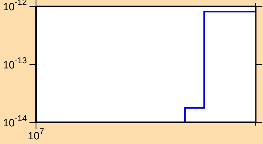
\sigma vs. E for ^{180}\text{W} (mt 45)
