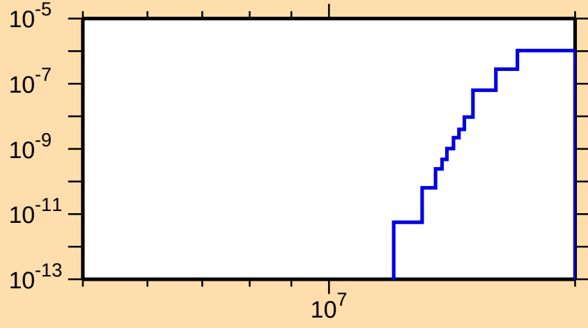
\sigma vs. E for ^{180}\text{W}(n,2n\alpha)
