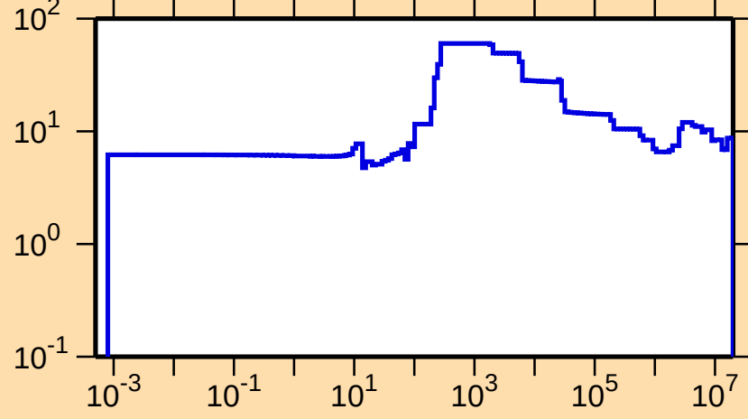
\Delta\sigma/\sigma vs. E for ^{180}\text{W}(n,\text{el.})
