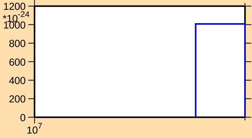
\sigma vs. E for ^{180}\text{W} (mt 11)
