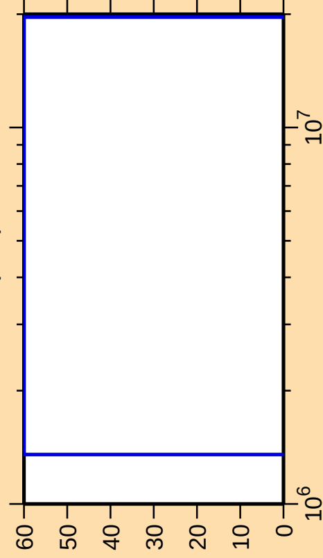
\Delta\sigma/\sigma vs. E for ^{180}\text{W}(n,\alpha)
