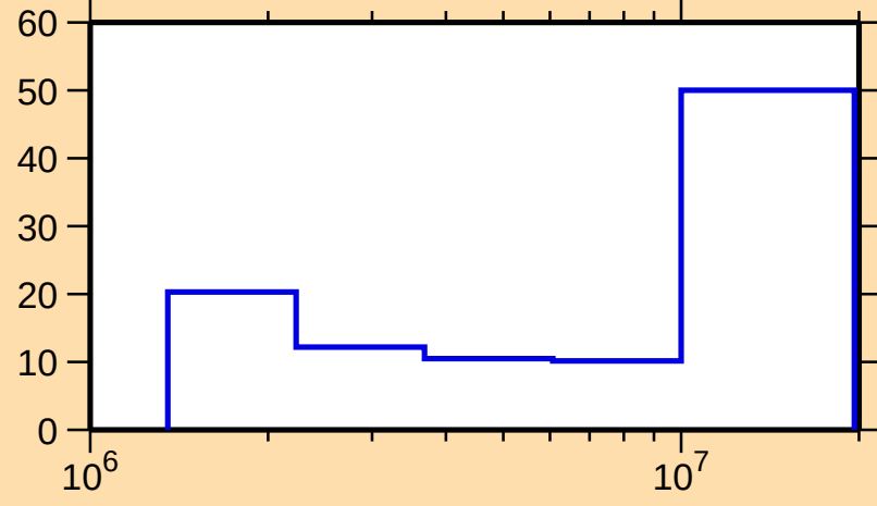
\Delta\sigma/\sigma vs. E for ^{180}\text{W}(n,\text{ncont.})
