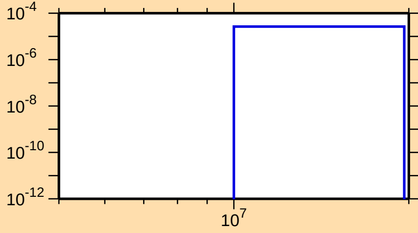
\sigma vs. E for ^{180}\text{W}(n,t)
