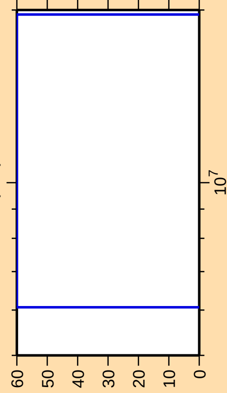
\Delta\sigma/\sigma vs. E for ^{180}\text{W}(n,d)
