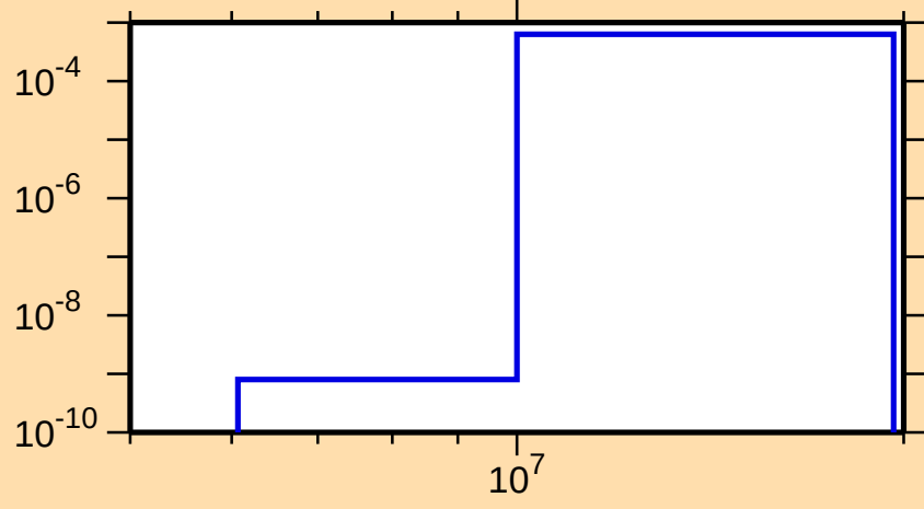
\sigma vs. E for ^{180}\text{W}(n,d)
