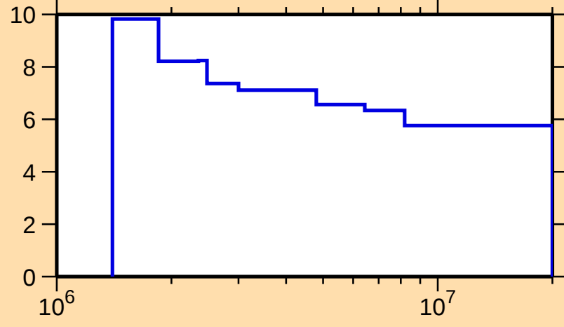
\Delta\sigma/\sigma vs. E for ^{180}\text{W}(\text{n},\text{nonel.})
