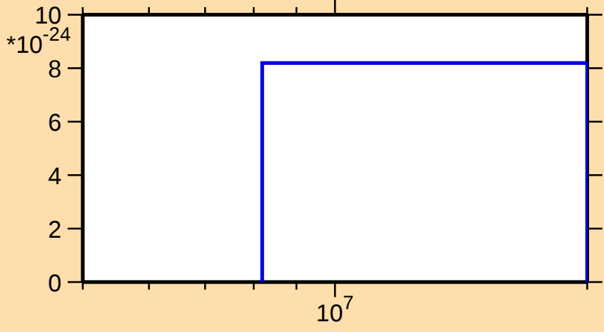
\sigma vs. E for ^{180}\text{W}(\text{mt 11})
