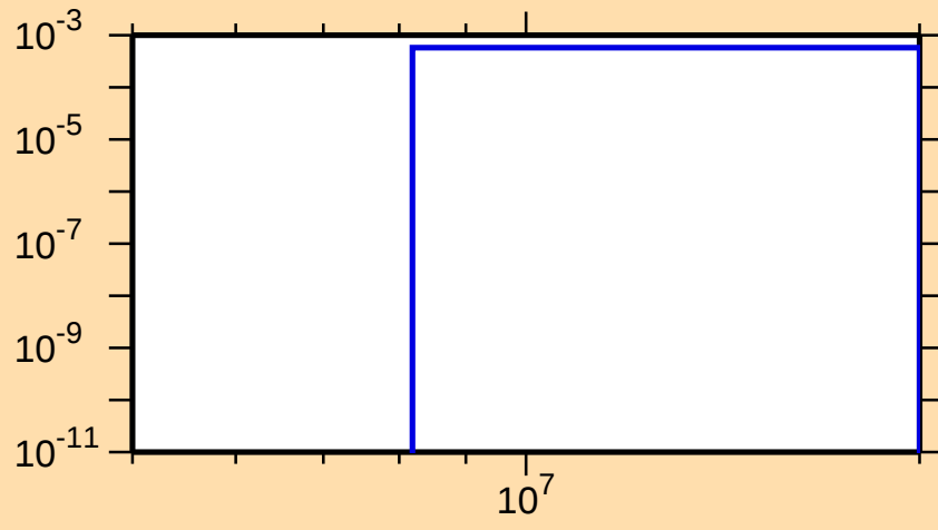
\sigma vs. E for ^{180}\text{W}(n,np)
