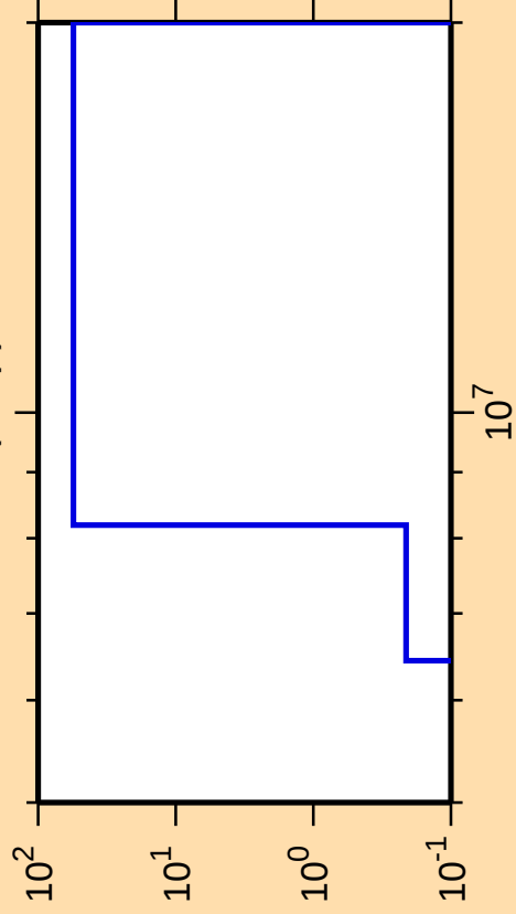
\Delta\sigma/\sigma vs. E for ^{180}\text{W}(n,np)
