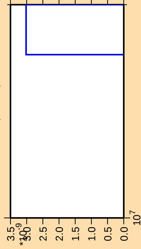
\Delta\sigma/\sigma vs. E for ^{183}\text{W} (mt 11)
