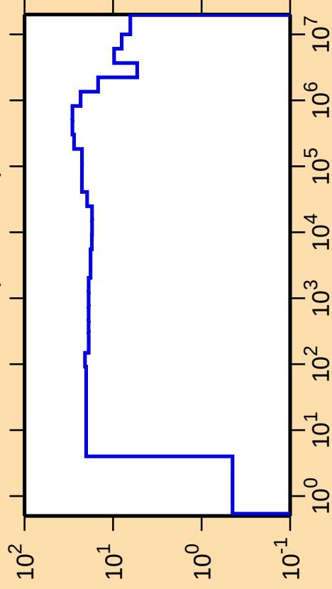
\Delta\sigma/\sigma vs. E for ^{183}\text{W}(\text{n,nonel.})
