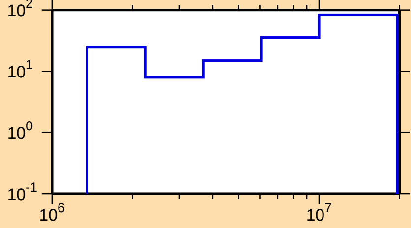
\Delta\sigma/\sigma vs. E for ^{183}\text{W}(n,ncont.)
