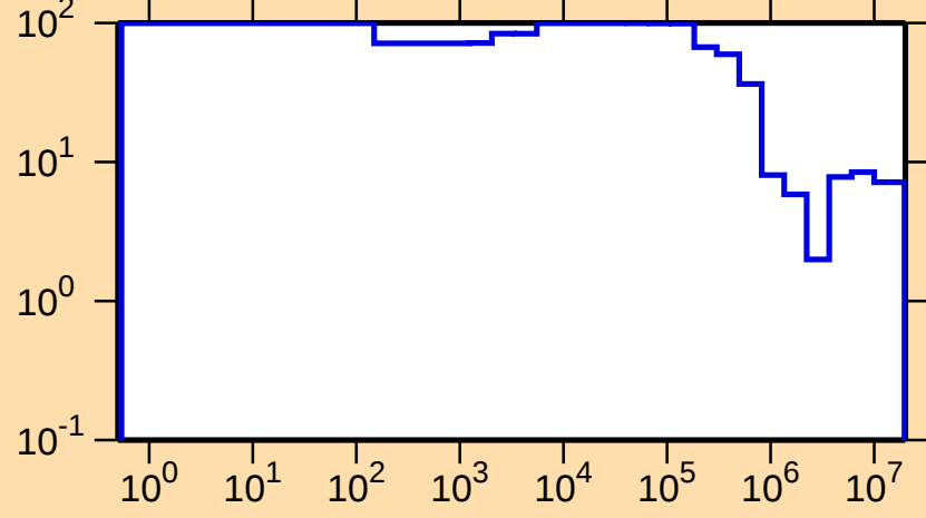
\Delta\sigma/\sigma vs. E for ^{183}\text{W}(\text{n,el.})
