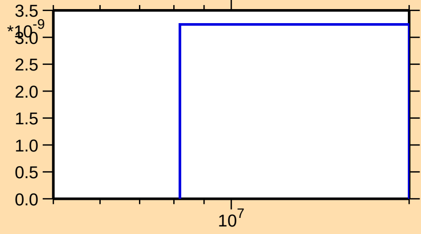
\sigma vs. E for ^{183}\text{W}(n,2np)
