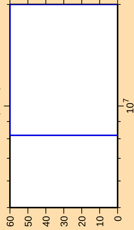
\Delta\sigma/\sigma vs. E for ^{183}\text{W}(\text{n},\text{nd})
