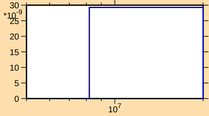
\sigma vs. E for ^{183}\text{W}(\text{n},\text{nd})
