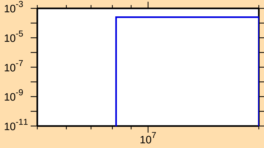
\sigma vs. E for ^{183}\text{W}(n,d)
