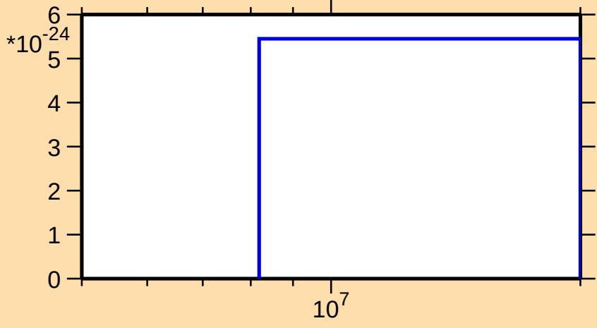
\sigma vs. E for ^{183}\text{W}(\text{mt 11})
