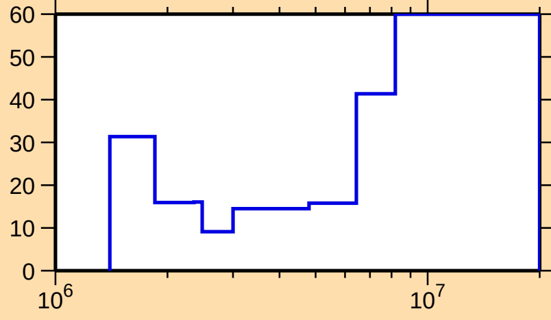
\Delta\sigma/\sigma vs. E for ^{183}\text{W}(n,n\text{cont.})
