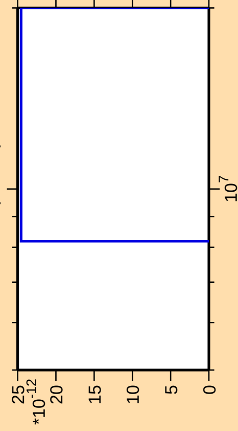
\Delta\sigma/\sigma vs. E for ^{183}\text{W}(\text{mt 11})
