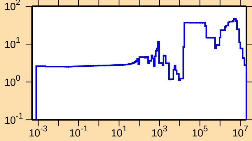
\Delta\sigma/\sigma vs. E for ^{184}\text{W}(\text{n},\text{tot.})
