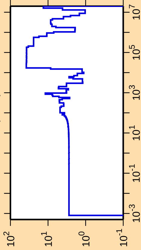
\Delta\sigma/\sigma vs. E for ^{184}\text{W}(\text{n},\text{el.})
