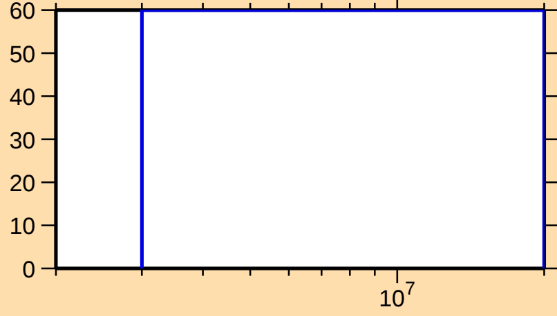
\Delta\sigma/\sigma vs. E for ^{184}\text{W}(\text{n},\text{ncont.})
