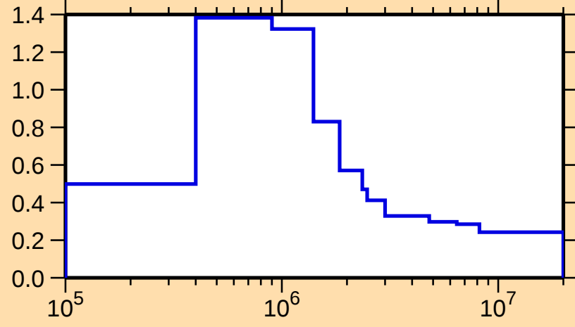
\sigma vs. E for ^{184}\text{W}(n,n_1)
