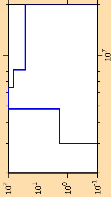
\Delta\sigma/\sigma vs. E for ^{184}\text{W}(\text{n},\text{p})
