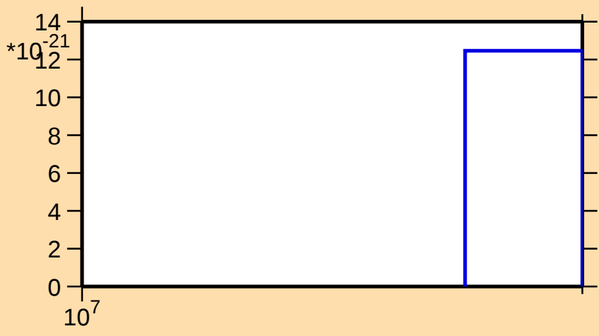
\sigma vs. E for ^{185}\text{W} (mt 11)
