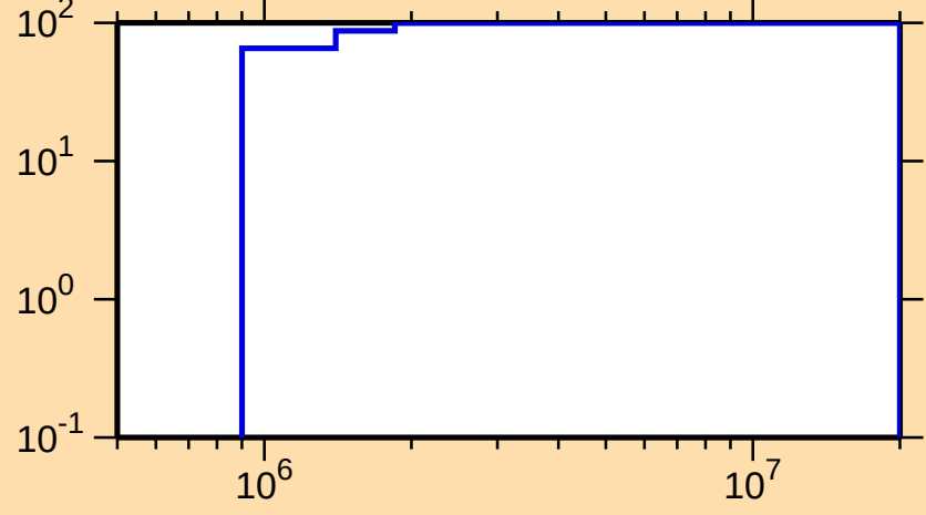
\Delta\sigma/\sigma vs. E for ^{185}\text{W}(n,n_1)
