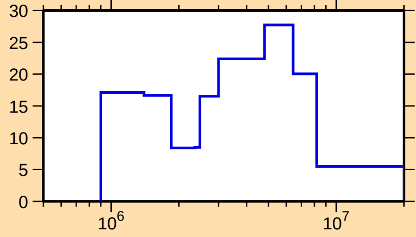
\Delta\sigma/\sigma vs. E for ^{185}\text{W}(\text{n},\text{el.})
