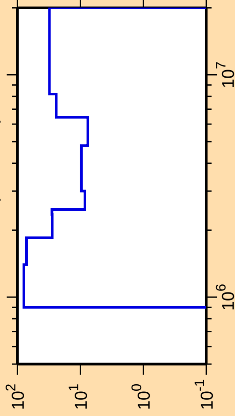
\Delta\sigma/\sigma vs. E for ^{185}\text{W}(\text{n},\text{ncont.})
