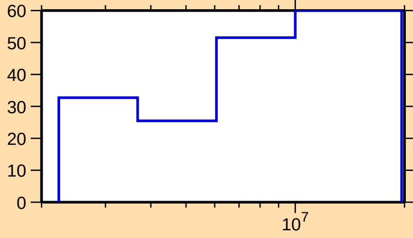
\Delta\sigma/\sigma vs. E for ^{188}\text{W}(n,n\text{cont.})
