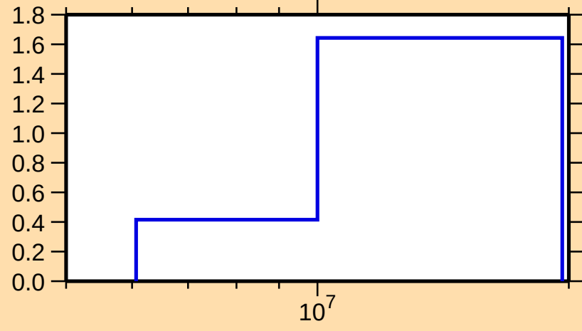
\sigma vs. E for ^{188}\text{W}(n,2n)
