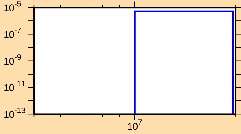
\sigma vs. E for ^{188}\text{W}(n,t)
