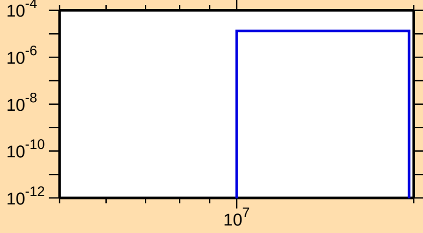
\sigma vs. E for ^{188}\text{W}(n,d)
