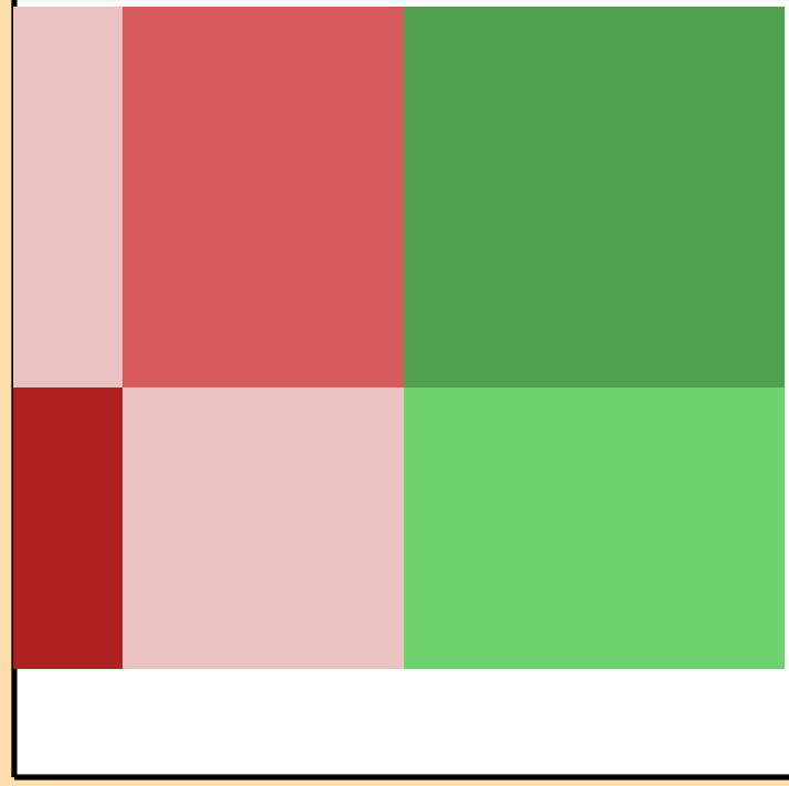
\Delta\sigma/\sigma vs. E for ^{188}\text{W}(n,\gamma)
