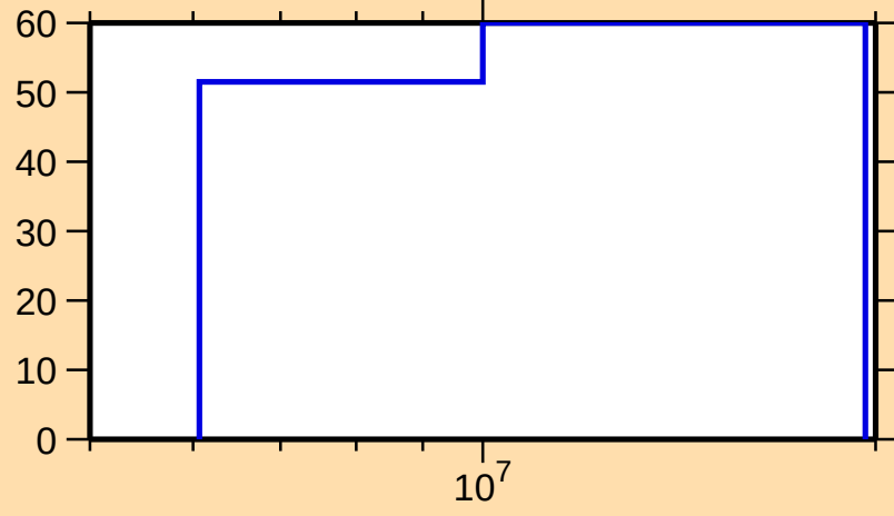
\Delta\sigma/\sigma vs. E for ^{188}\text{W}(\text{n,ncont.})
