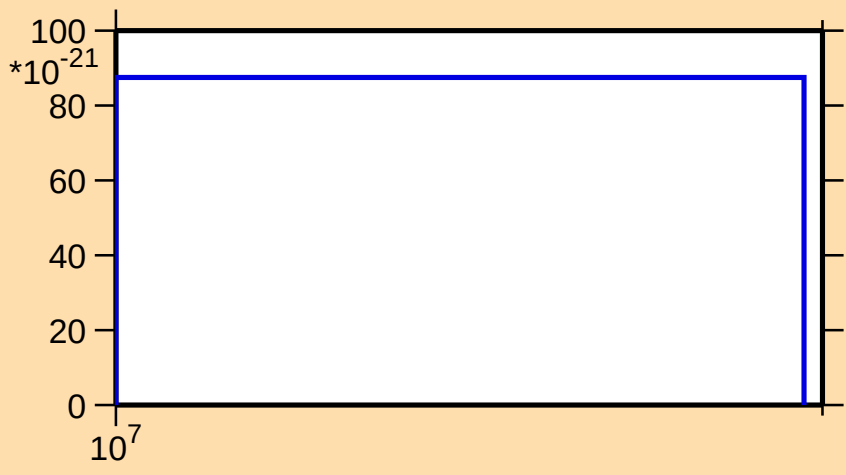
\sigma vs. E for ^{188}\text{W} (mt 11)
