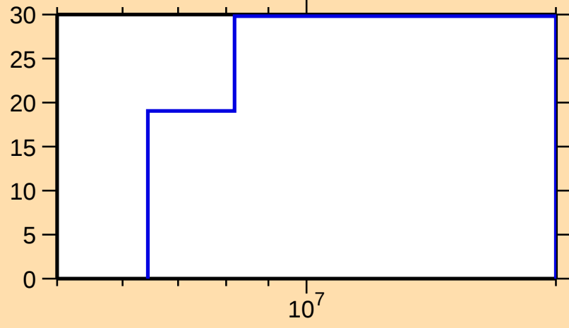
\Delta\sigma/\sigma vs. E for ^{188}\text{W}(\text{n},2\text{n})
