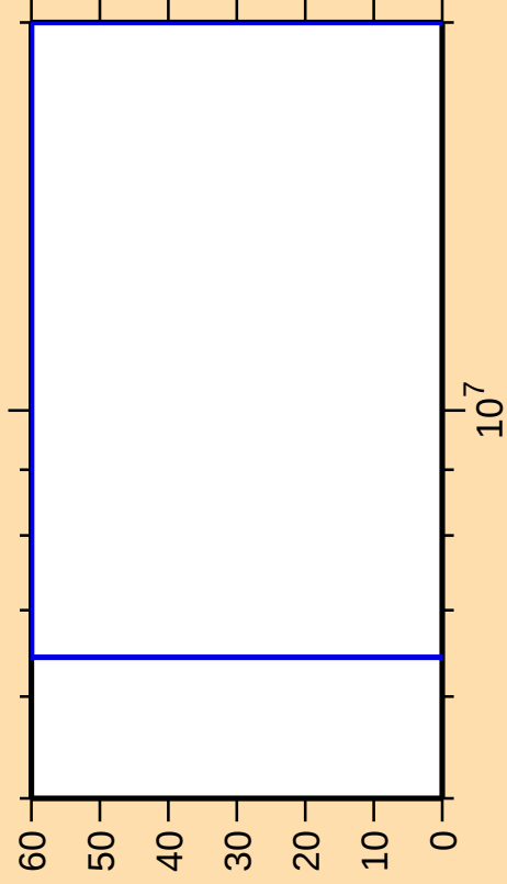
\Delta\sigma/\sigma vs. E for ^{188}\text{W}(\text{n},\text{ncont.})
