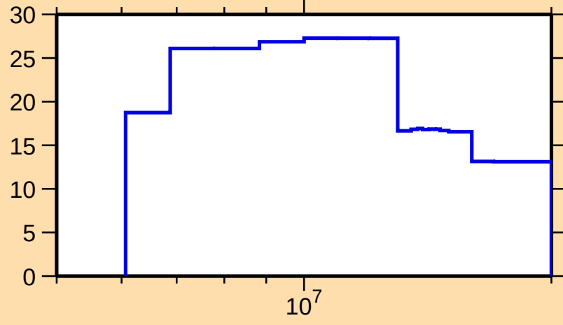
\Delta\sigma/\sigma vs. E for ^{190}\text{W}(\text{n,el.})
