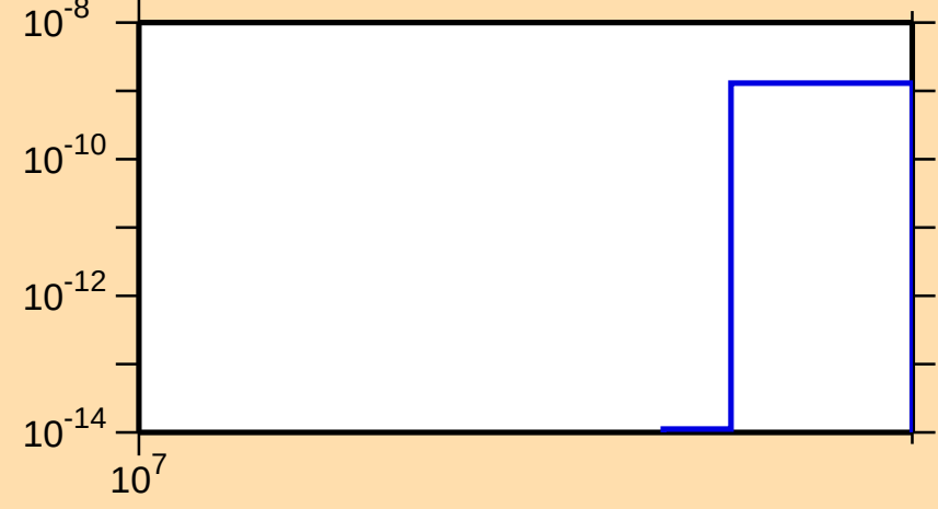
\sigma vs. E for ^{190}\text{W}(\text{n},\text{nd})
