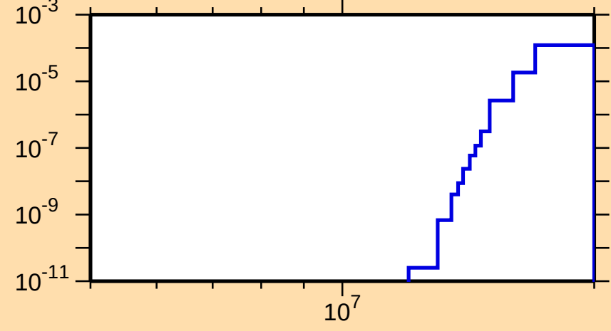
\sigma vs. E for ^{190}\text{W}(n,np)
