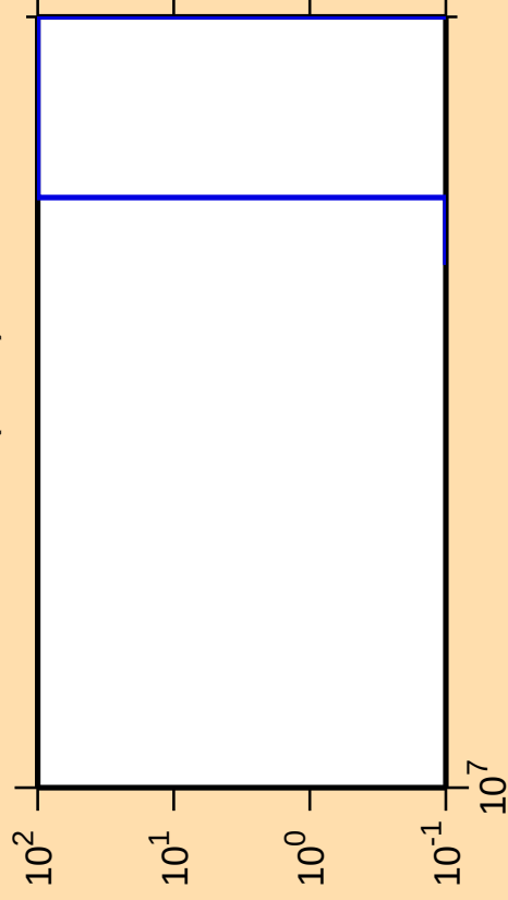
\Delta\sigma/\sigma vs. E for ^{190}\text{W}(\text{n},\text{nd})
