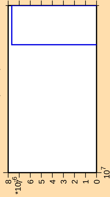
\Delta\sigma/\sigma vs. E for ^{190}\text{W} (mt 11)
