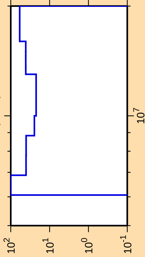
\Delta\sigma/\sigma vs. E for ^{190}\text{W}(n,2n)
