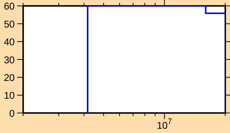
\Delta\sigma/\sigma vs. E for ^{190}\text{W}(n,\gamma)
