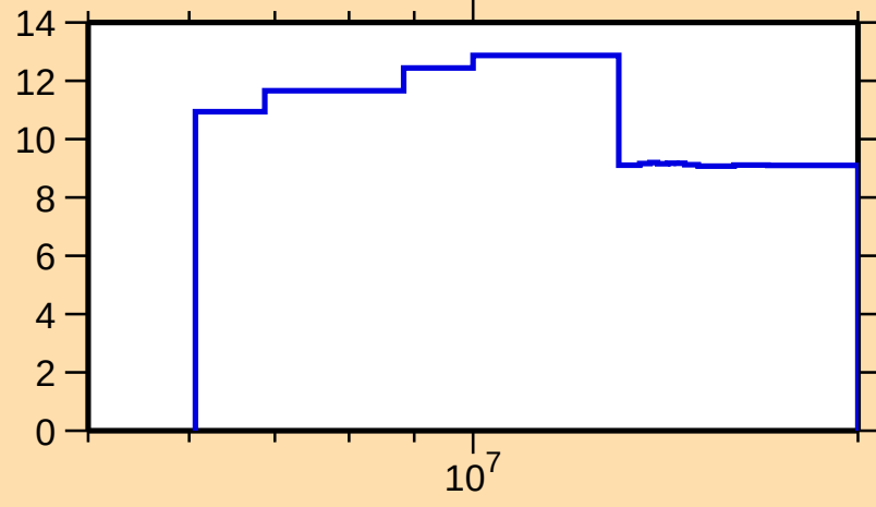
\Delta\sigma/\sigma vs. E for ^{190}\text{W}(\text{n,tot.})
