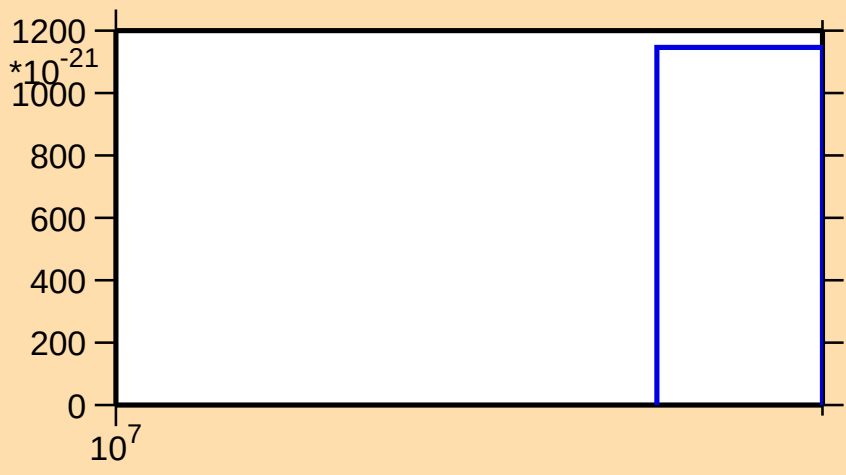
\sigma vs. E for ^{190}\text{W} (mt 11)
