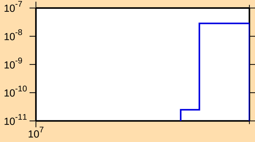
\sigma vs. E for ^{190}\text{W}(n,nt)
