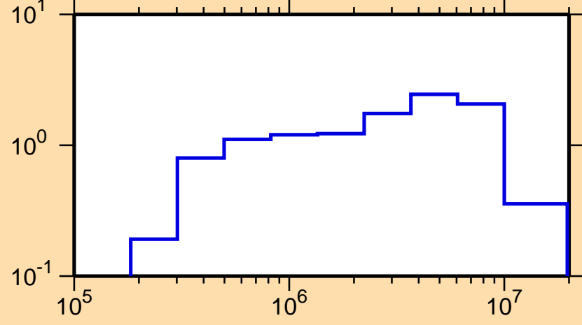
\sigma vs. E for ^{190}\text{W}(n,\text{inel.})
