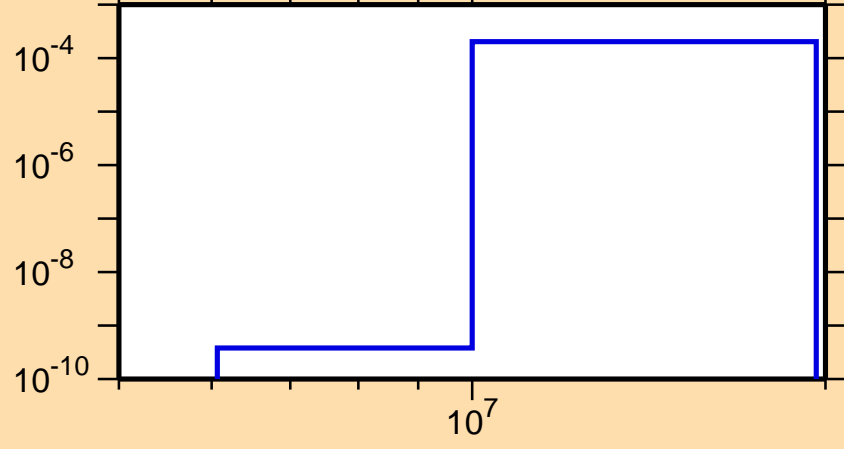
\sigma vs. E for ^{190}\text{W}(n,p)
