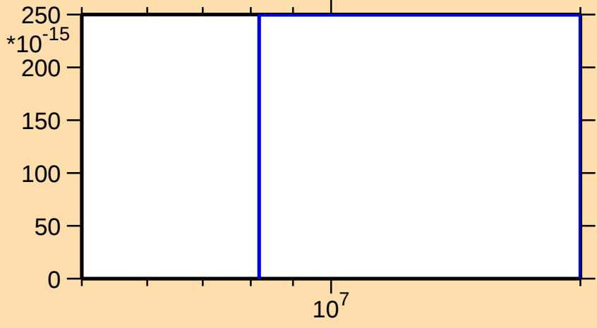
\sigma vs. E for ^{190}\text{W}(n,2np)
