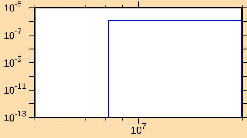
\sigma vs. E for ^{190}\text{W}(n,t)
