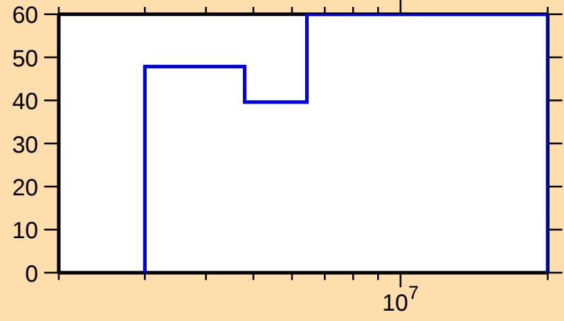
\Delta\sigma/\sigma vs. E for ^{190}\text{W}(n,\text{ncont.})
