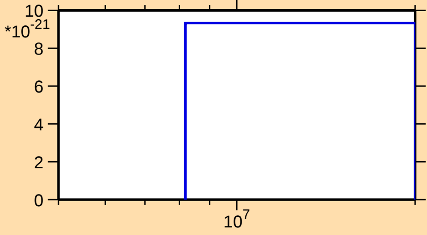
\sigma vs. E for ^{190}\text{W}(\text{mt 11})
