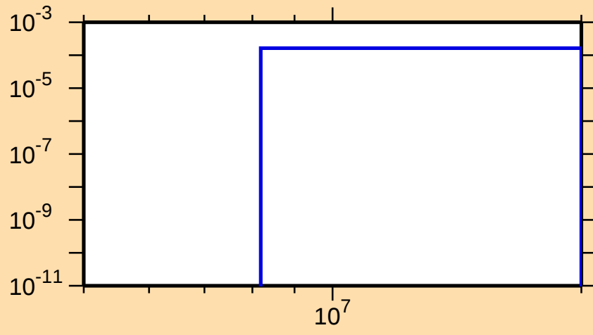
\sigma vs. E for ^{190}\text{W}(n,p)
