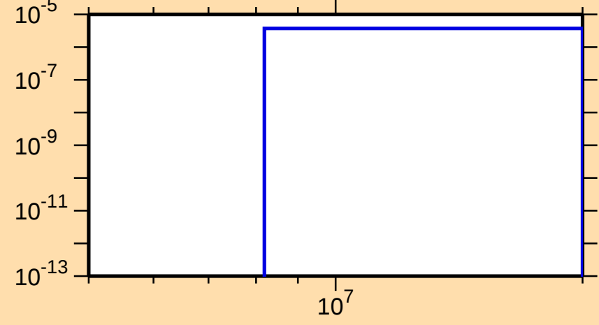
\sigma vs. E for ^{190}\text{W}(n,d)
