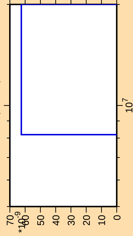
\Delta\sigma/\sigma vs. E for ^{190}\text{W}(\text{mt 11})
