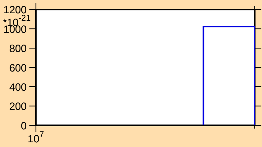
\sigma vs. E for ^{191}\text{W} (mt 11)
