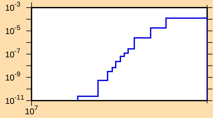
\sigma vs. E for ^{191}\text{W}(n,np)
