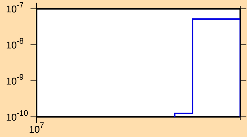
\sigma vs. E for ^{191}\text{W}(\text{n},\text{nd})
