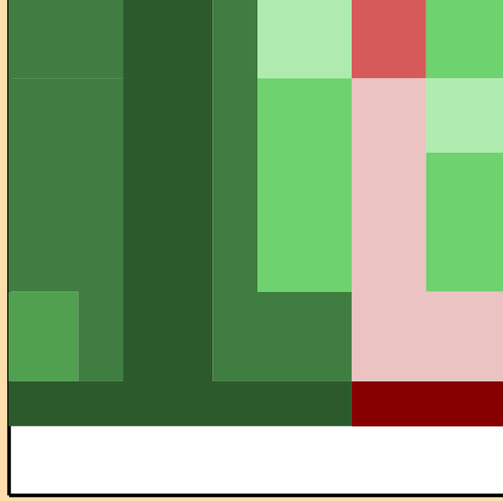
\Delta\sigma/\sigma vs. E for ^{191}\text{W}(n,\text{tot.})
