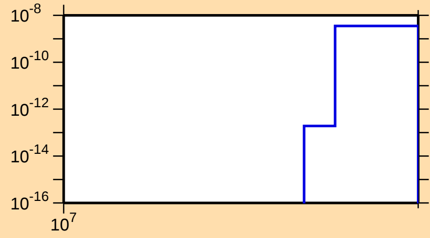
\sigma vs. E for ^{191}\text{W}(n,2np)
