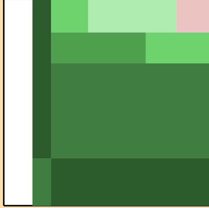
\Delta\sigma/\sigma vs. E for ^{191}\text{W}(n,p)
