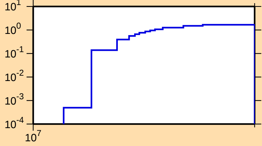
\sigma vs. E for ^{191}\text{W}(n,3n)
