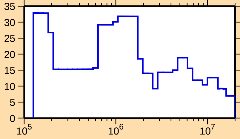
\Delta\sigma/\sigma vs. E for ^{191}\text{W}(\text{n},\text{el.})
