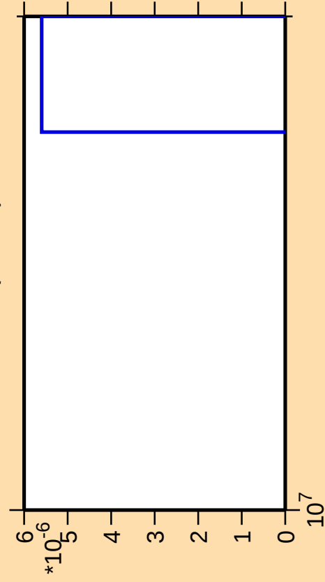
\Delta\sigma/\sigma vs. E for ^{191}\text{W} (mt 11)
