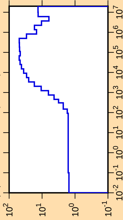
\Delta\mu/\mu vs. E for ^{191}\text{W}(\text{mt251})
