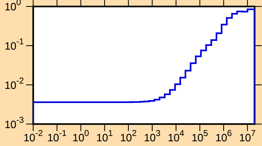
\mu vs. E for ^{191}\text{W}(\text{mt251})
