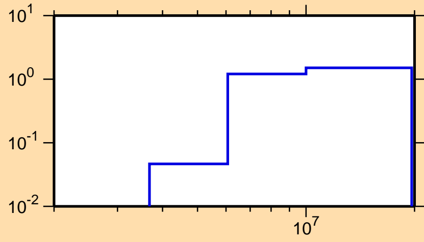
\sigma vs. E for ^{191}\text{W}(n,2n)
