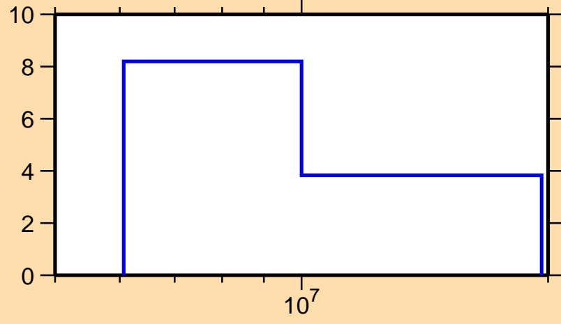
\Delta\sigma/\sigma vs. E for ^{191}\text{W}(n,\text{tot.})
