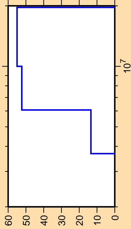
\Delta\sigma/\sigma vs. E for ^{191}\text{W}(n,n\text{cont.})
