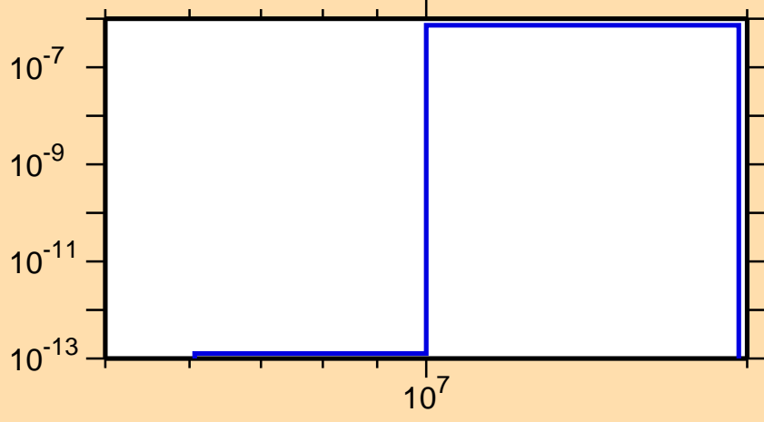
\sigma vs. E for ^{191}\text{W}(n,n\alpha)
