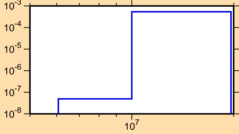
\sigma vs. E for ^{191}\text{W}(n,p)
