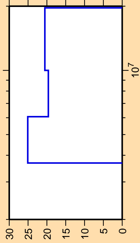
\Delta\sigma/\sigma vs. E for ^{191}\text{W}(n,n_1)
