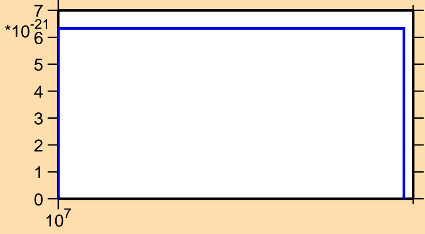
\sigma vs. E for ^{191}\text{W} (mt 11)
