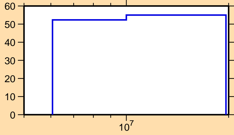
\Delta\sigma/\sigma vs. E for ^{191}\text{W}(n,ncont.)
