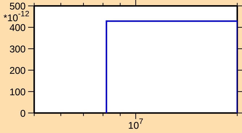
\sigma vs. E for ^{191}\text{W}(n,\text{nd})
