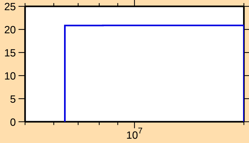
\Delta\sigma/\sigma vs. E for ^{191}\text{W}(n,n_1)
