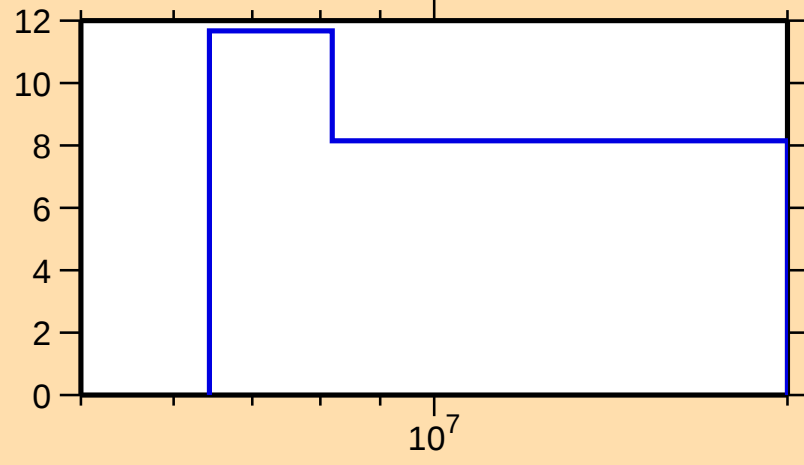
\Delta\sigma/\sigma vs. E for ^{191}\text{W}(\text{n,el.})
