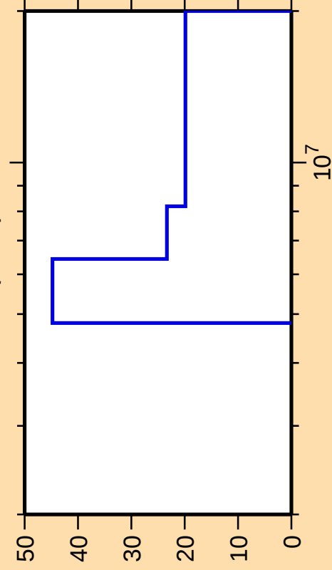
\Delta\sigma/\sigma vs. E for ^{191}\text{W}(n,2n)
