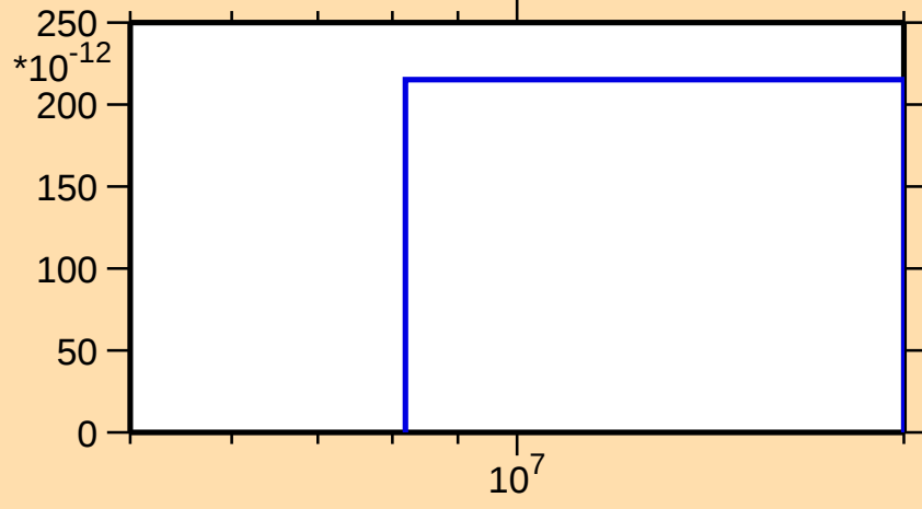
\sigma vs. E for ^{191}\text{W}(n,nt)
