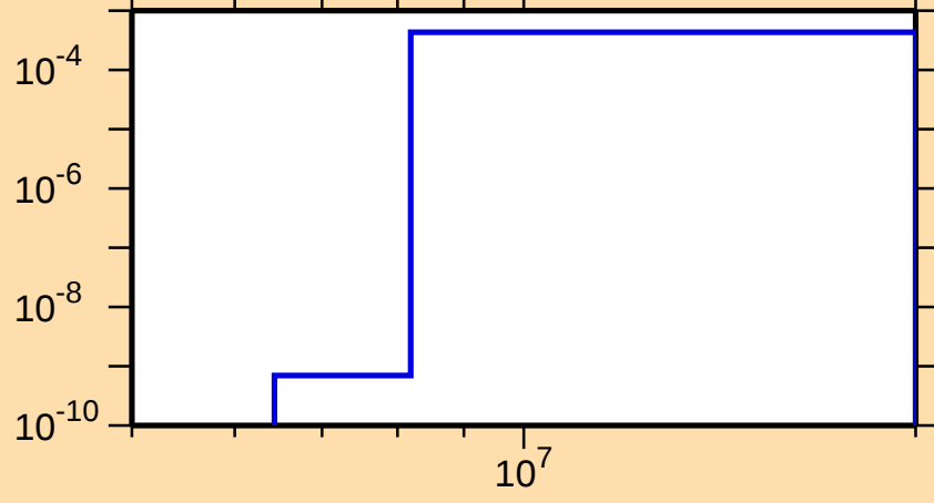
\sigma vs. E for ^{191}\text{W}(n,p)
