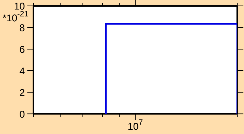
\sigma vs. E for ^{191}\text{W}(\text{mt 11})
