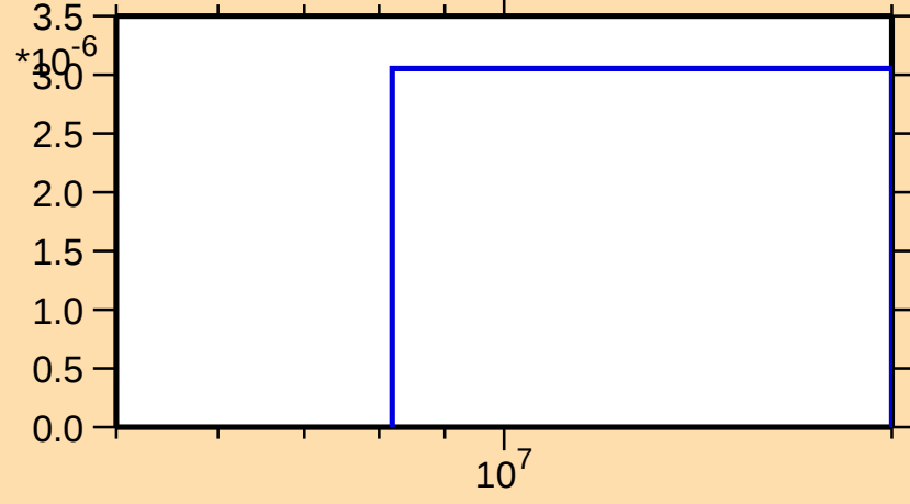
\sigma vs. E for ^{191}\text{W}(n,t)
