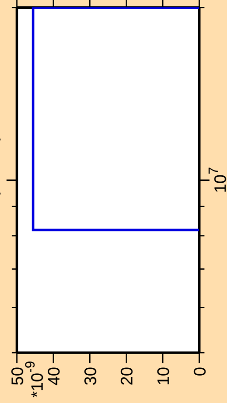
\Delta\sigma/\sigma vs. E for ^{191}\text{W}(\text{mt 11})
