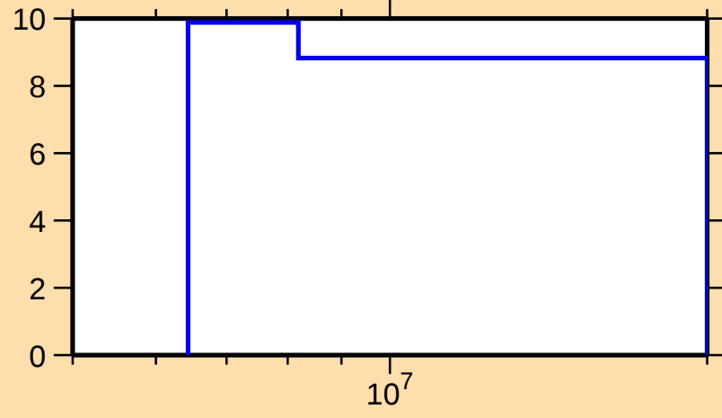
\Delta\sigma/\sigma vs. E for ^{191}\text{W}(\text{n,nonel.})
