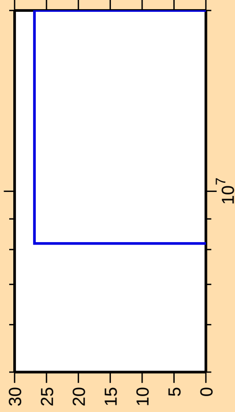
\Delta\sigma/\sigma vs. E for ^{191}\text{W}(n,3n)
