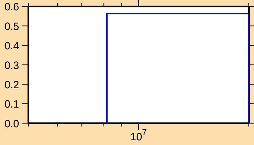
\sigma vs. E for ^{191}\text{W}(n,3n)
