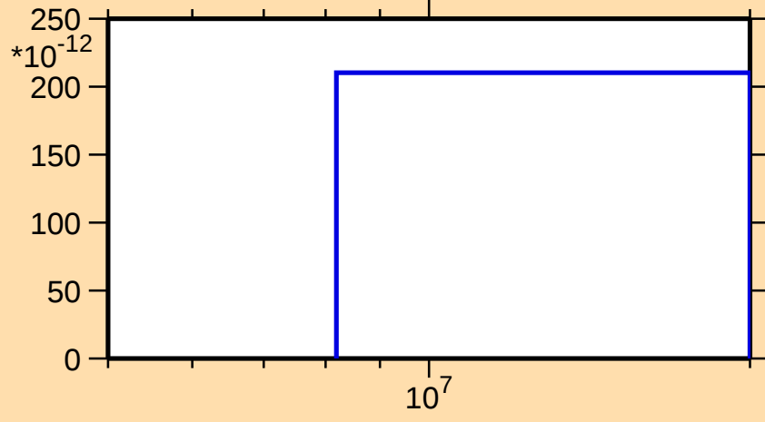
\sigma vs. E for ^{191}\text{W}(n,2n\alpha)
