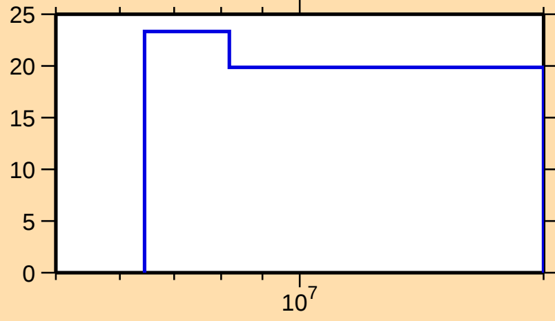
\Delta\sigma/\sigma vs. E for ^{191}\text{W}(n,2n)
