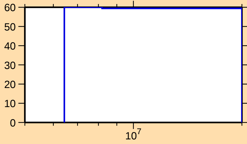
\Delta\sigma/\sigma vs. E for ^{191}\text{W}(n,n\text{cont.})
