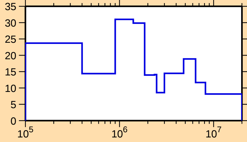
\Delta\sigma/\sigma vs. E for ^{191}\text{W}(n,\text{el.})
