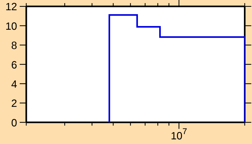
\Delta\sigma/\sigma vs. E for ^{191}\text{W}(n,\text{nonel.})
