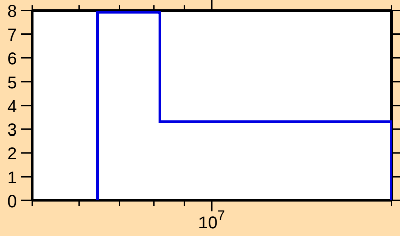
\Delta\sigma/\sigma vs. E for ^{191}\text{W}(\text{n,tot.})
