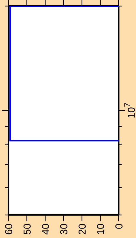
\Delta\sigma/\sigma vs. E for ^{191}\text{W}(n,2np)
