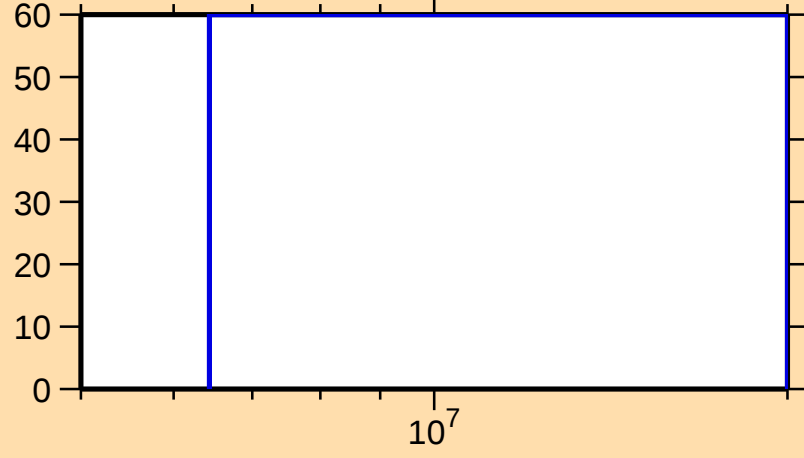
\Delta\sigma/\sigma vs. E for ^{191}\text{W}(n,\gamma)
