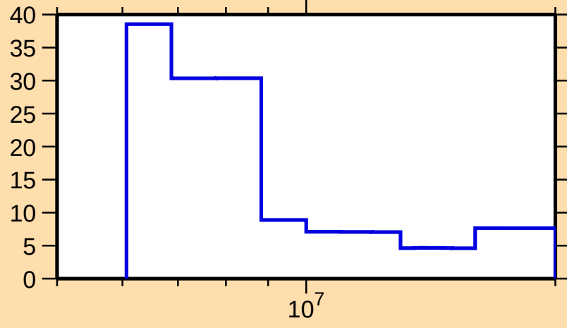
\Delta\sigma/\sigma vs. E for ^{193}\text{W}(\text{n,el.})
