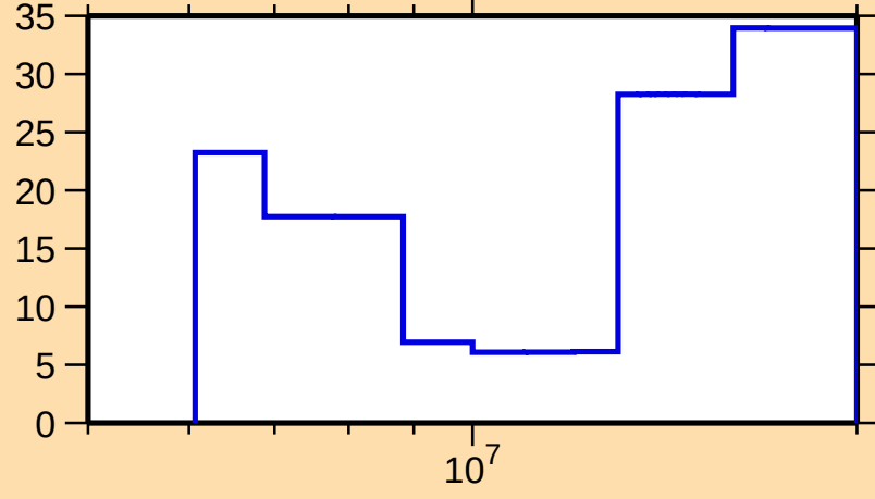
\Delta\sigma/\sigma vs. E for ^{193}\text{W}(n,2n)
