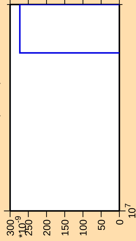
\Delta\sigma/\sigma vs. E for ^{193}\text{W} (mt 11)
