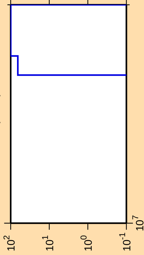
\Delta\sigma/\sigma vs. E for ^{193}\text{W}(\text{n},\text{nd})
