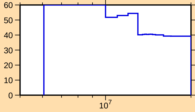
\Delta\sigma/\sigma vs. E for ^{193}\text{W}(n,\text{ncont.})
