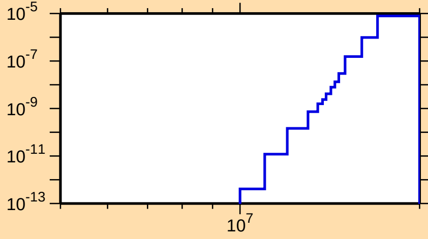
\sigma vs. E for ^{193}\text{W}(n,n\alpha)
