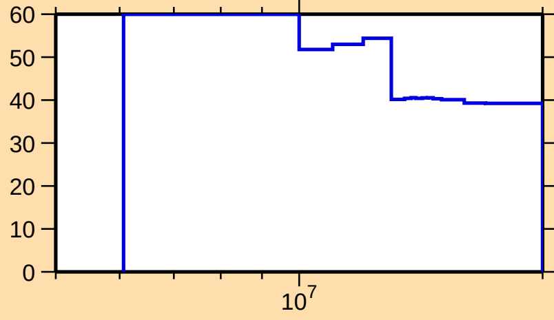
\Delta\sigma/\sigma vs. E for ^{193}\text{W}(n,n\text{cont.})
