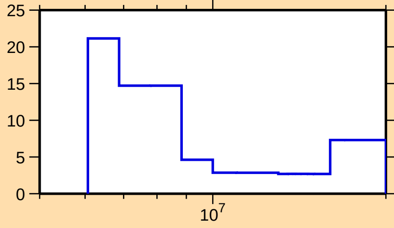
\Delta\sigma/\sigma vs. E for ^{193}\text{W}(\text{n,tot.})
