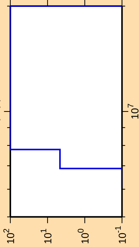
\Delta\sigma/\sigma vs. E for ^{193}\text{W}(\text{n,p})
