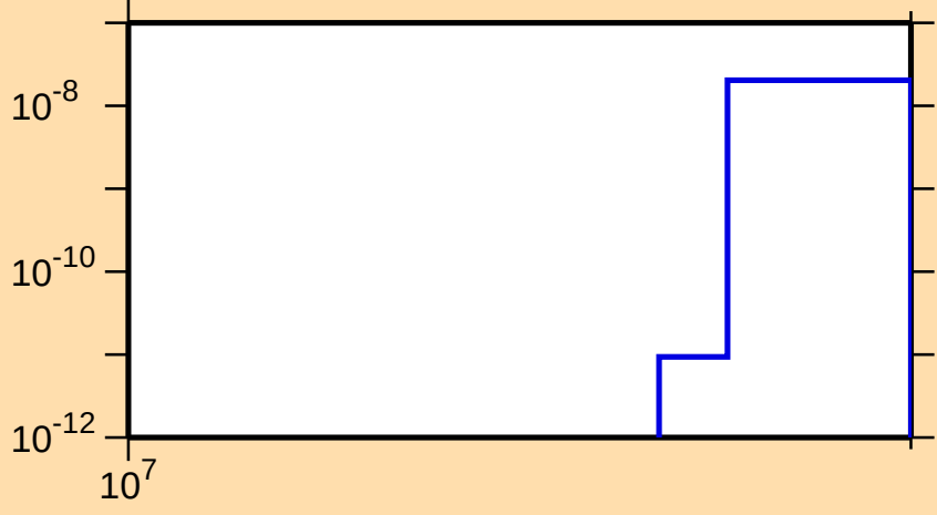
\sigma vs. E for ^{193}\text{W}(\text{n},\text{nd})
