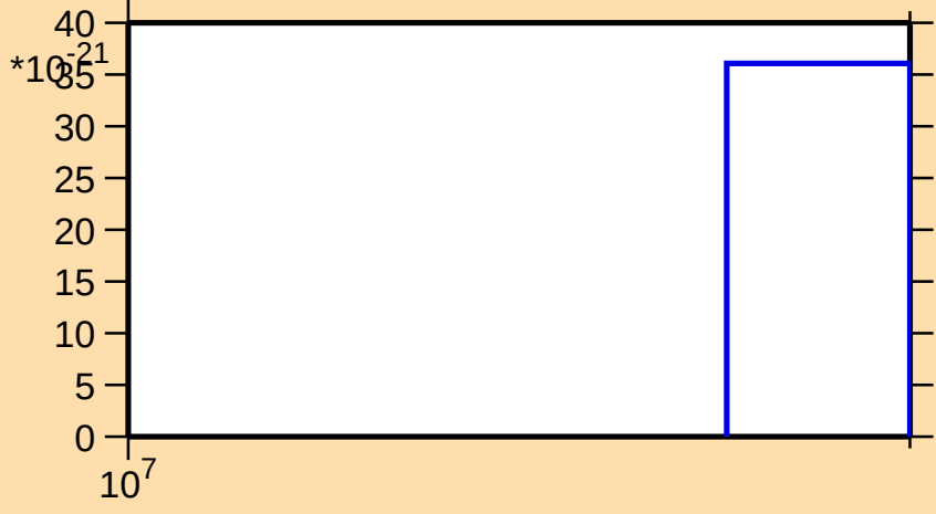
\sigma vs. E for ^{193}\text{W} (mt 11)
