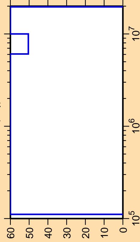
\Delta\sigma/\sigma vs. E for ^{193}\text{W}(n,\gamma)
