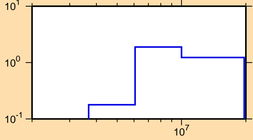
\sigma vs. E for ^{193}\text{W}(n,2n)
