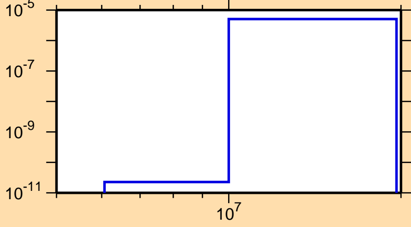
\sigma vs. E for ^{193}\text{W}(n,\alpha)
