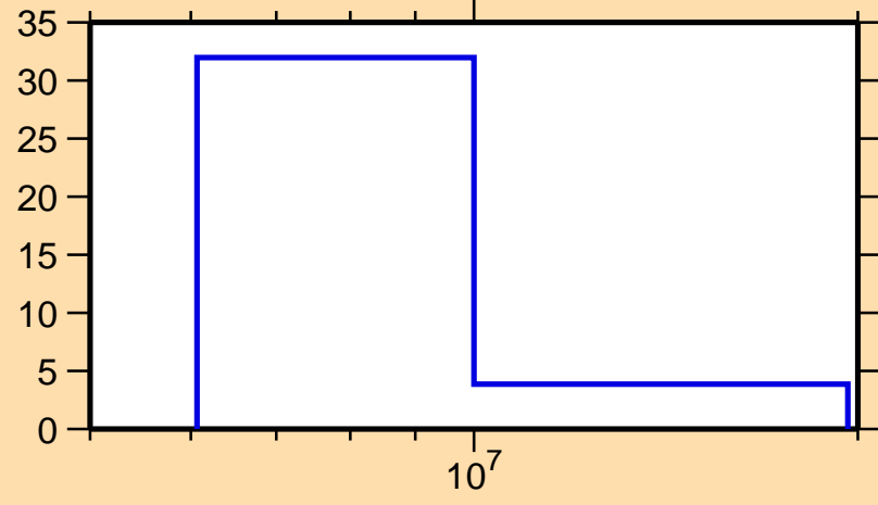
\Delta\sigma/\sigma vs. E for ^{193}\text{W}(n,el.)
