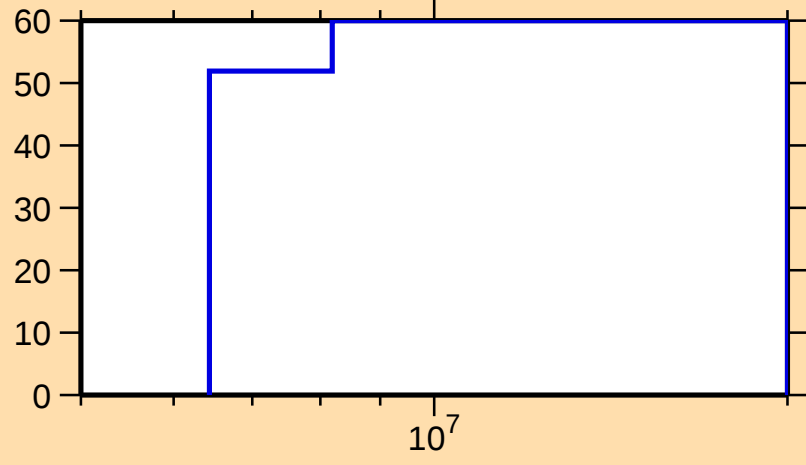
\Delta\sigma/\sigma vs. E for ^{193}\text{W}(n,\gamma)
