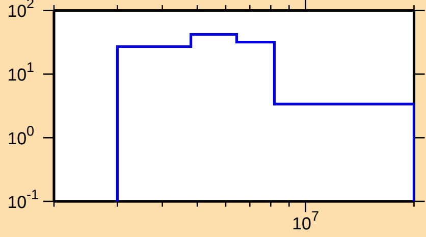
\Delta\sigma/\sigma vs. E for ^{193}\text{W}(n,\text{el.})
