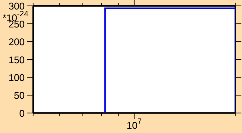
\sigma vs. E for ^{193}\text{W}(\text{mt 11})
