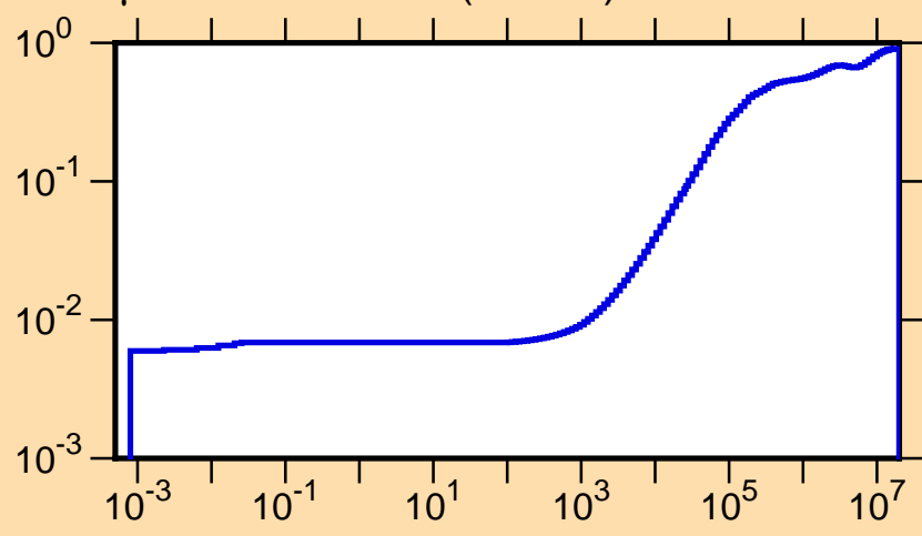
\mu vs. E for ^{114}\text{Xe}(\text{mt251})
