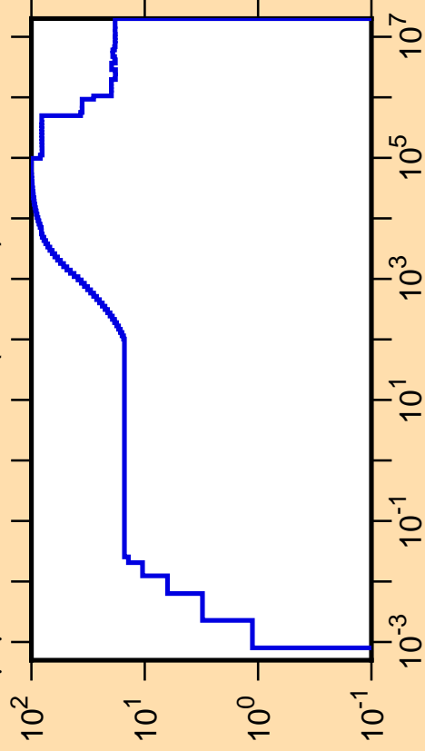
\Delta\mu/\mu vs. E for ^{114}\text{Xe}(\text{mt251})
