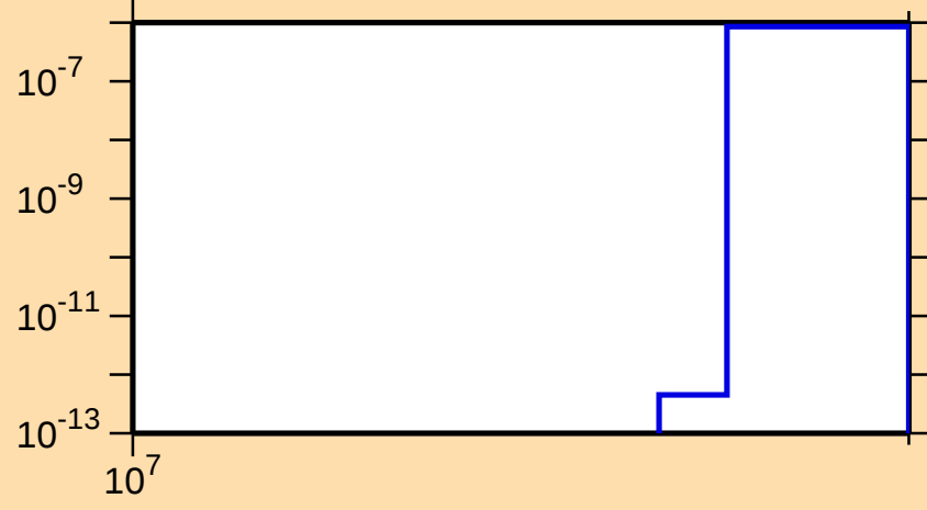
\sigma vs. E for ^{114}\text{Xe}(n,2np)
