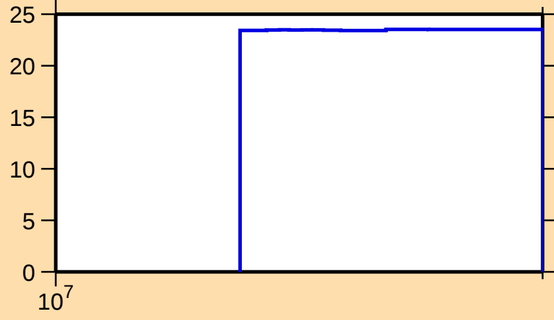
\Delta\sigma/\sigma vs. E for ^{114}\text{Xe}(n,\text{nonel.})
