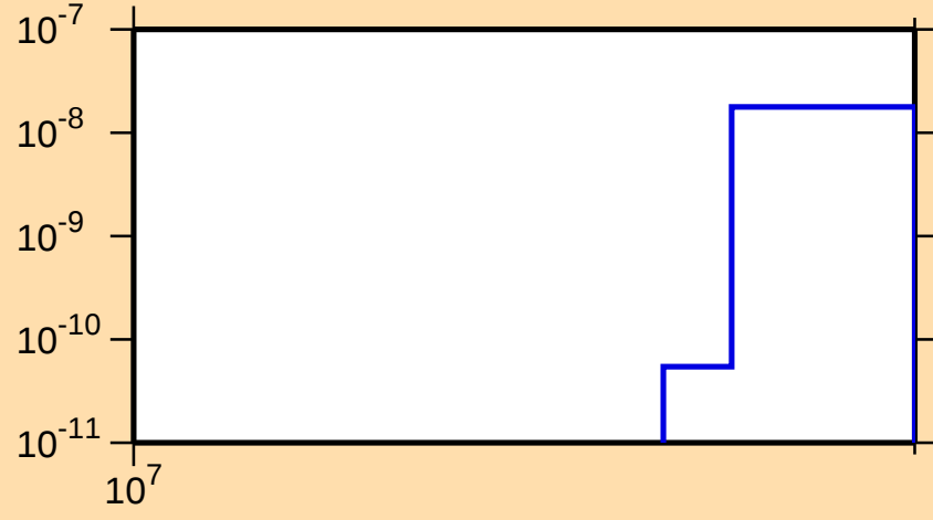
\sigma vs. E for ^{114}\text{Xe}(n,\text{nd})
