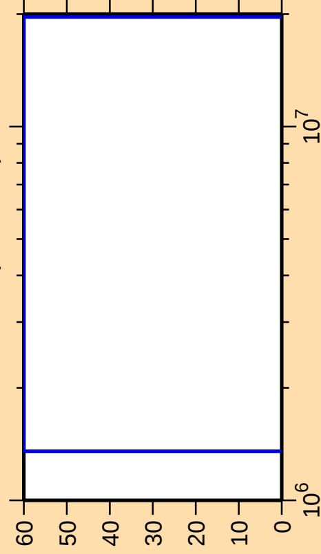
\Delta\sigma/\sigma vs. E for ^{114}\text{Xe}(n,\text{ncont.})
