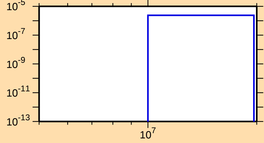
\sigma vs. E for ^{114}\text{Xe}(n,\text{pt})
