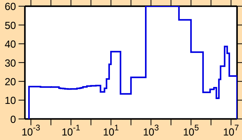
\Delta\sigma/\sigma vs. E for ^{114}\text{Xe}(n,\text{tot.})
