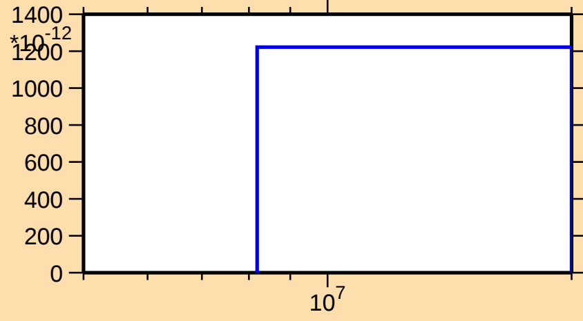
\sigma vs. E for ^{114}\text{Xe}(n,2n\alpha)
