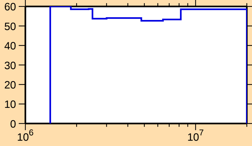
\Delta\sigma/\sigma vs. E for ^{114}\text{Xe}(n,\text{inel.})
