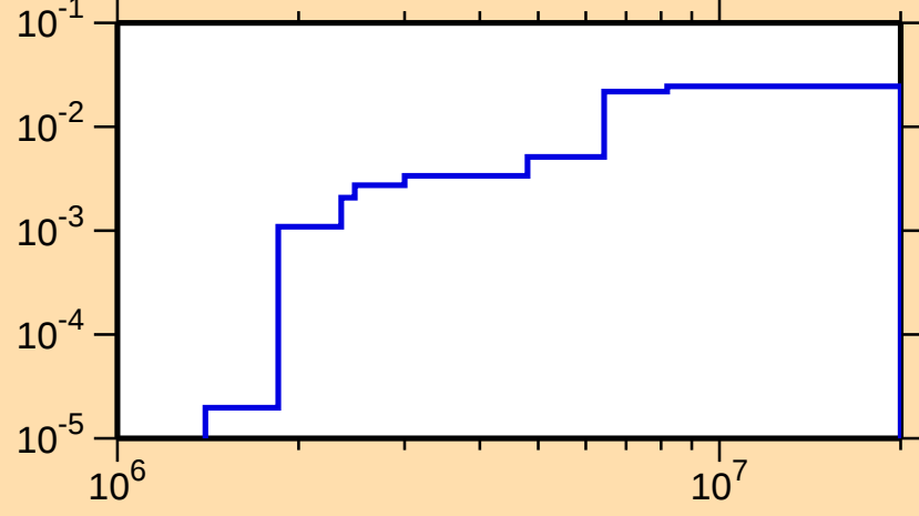
\sigma vs. E for ^{114}\text{Xe}(n,n\text{cont.})
