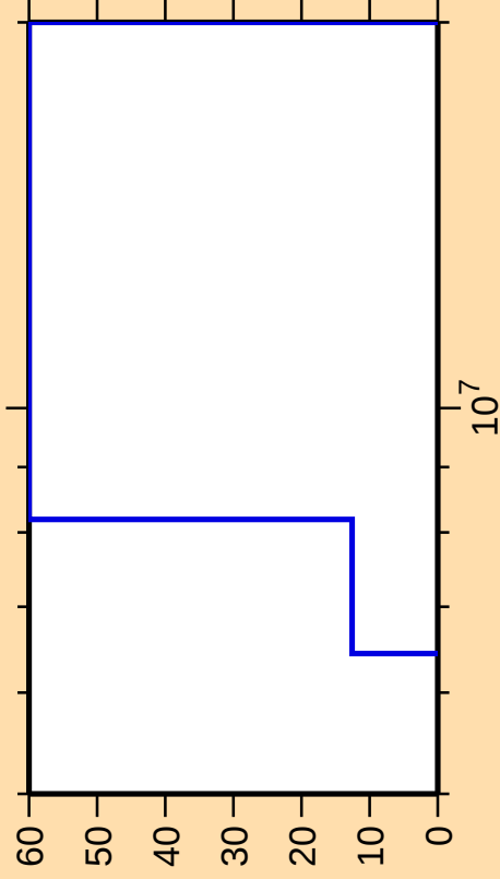
\Delta\sigma/\sigma vs. E for ^{114}\text{Xe}(\text{mt } 45)
