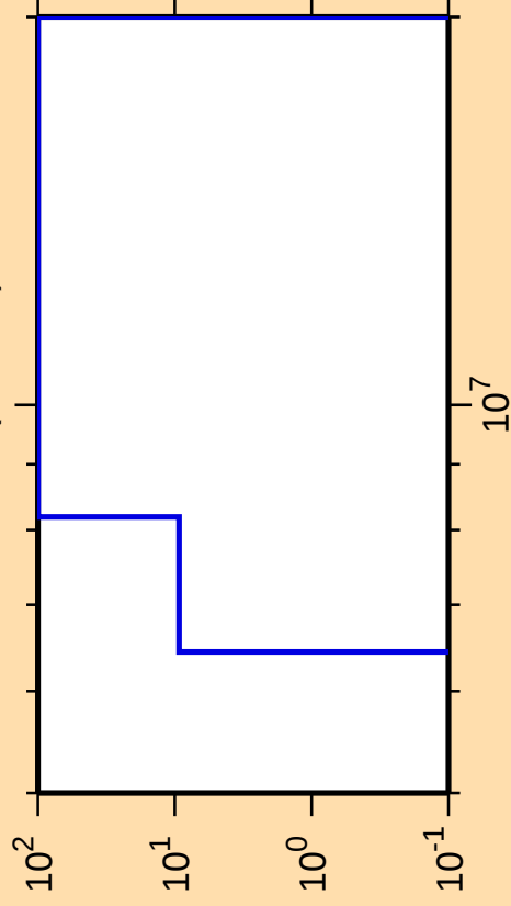
\Delta\sigma/\sigma vs. E for ^{114}\text{Xe}(\text{mt117})
