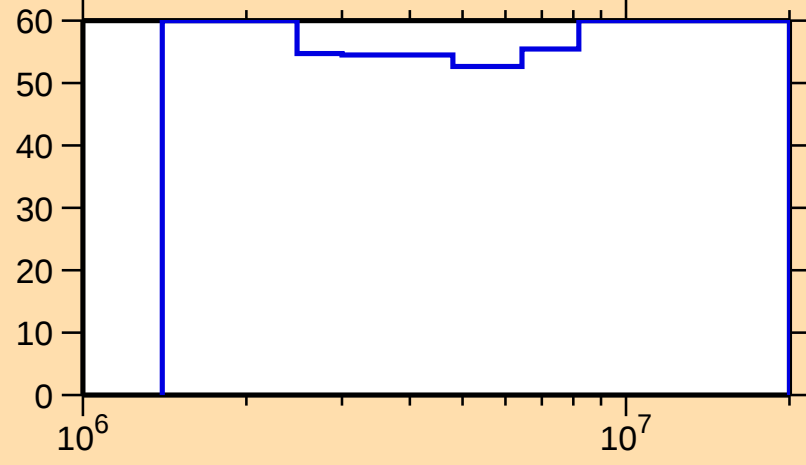
\Delta\sigma/\sigma vs. E for ^{114}\text{Xe}(n,n_1)
