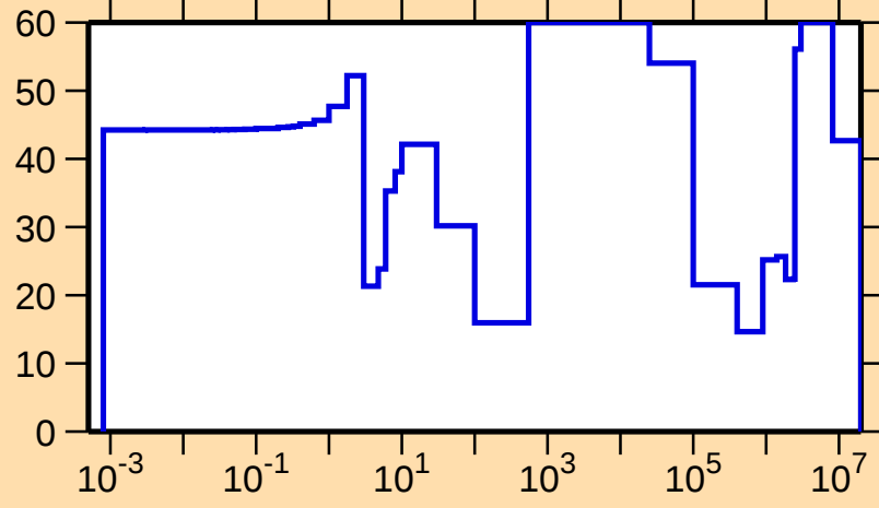
\Delta\sigma/\sigma vs. E for ^{114}\text{Xe}(n,\text{el.})
