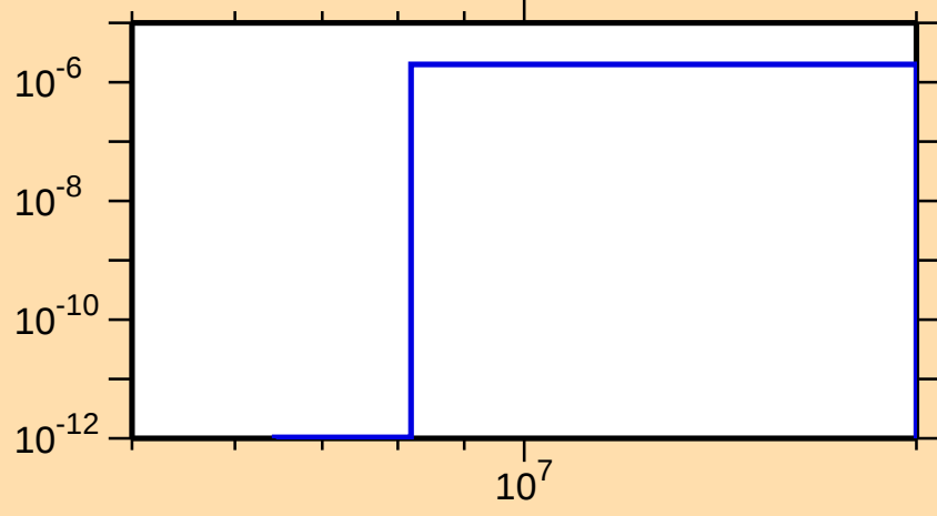
\sigma vs. E for ^{114}\text{Xe}(\text{mt117})
