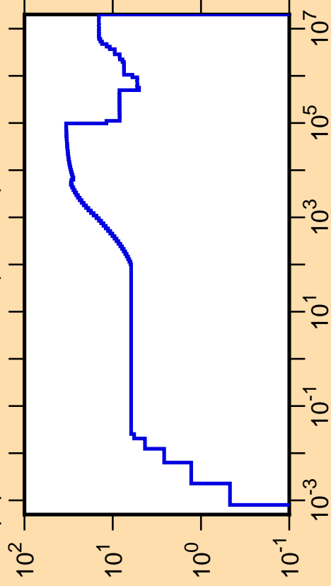
\Delta\mu/\mu vs. E for ^{117}\text{Xe}(\text{mt251})
