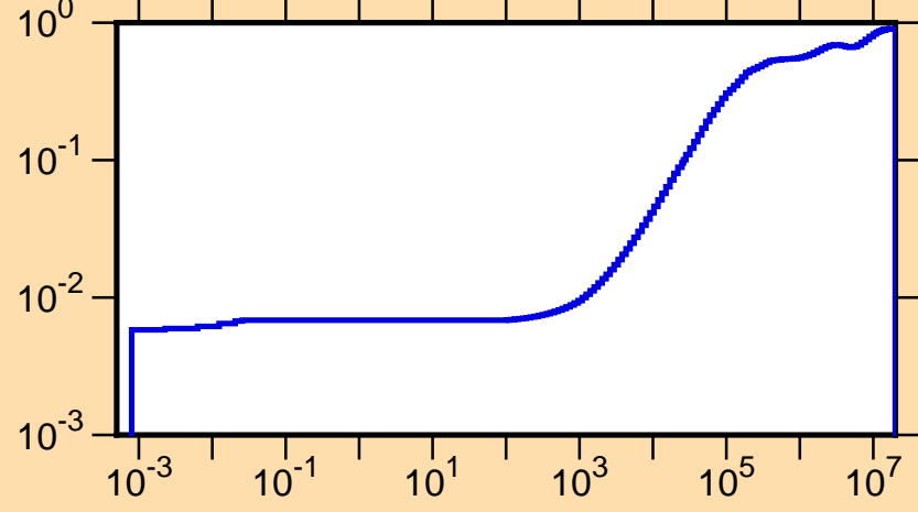
\mu vs. E for ^{117}\text{Xe}(\text{mt251})
