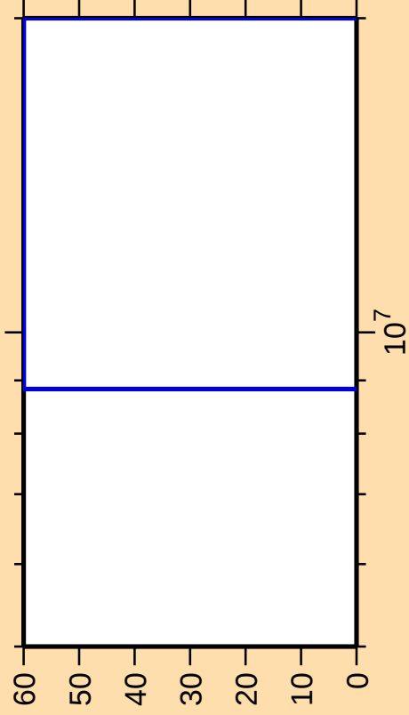
\Delta\sigma/\sigma vs. E for ^{117}\text{Xe}(n,n_1)
