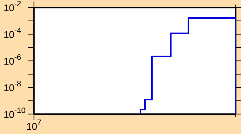
\sigma vs. E for ^{117}\text{Xe}(n,2np)
