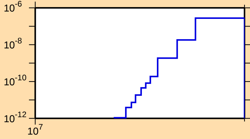
\sigma vs. E for ^{117}\text{Xe}(\text{mt } 34)
