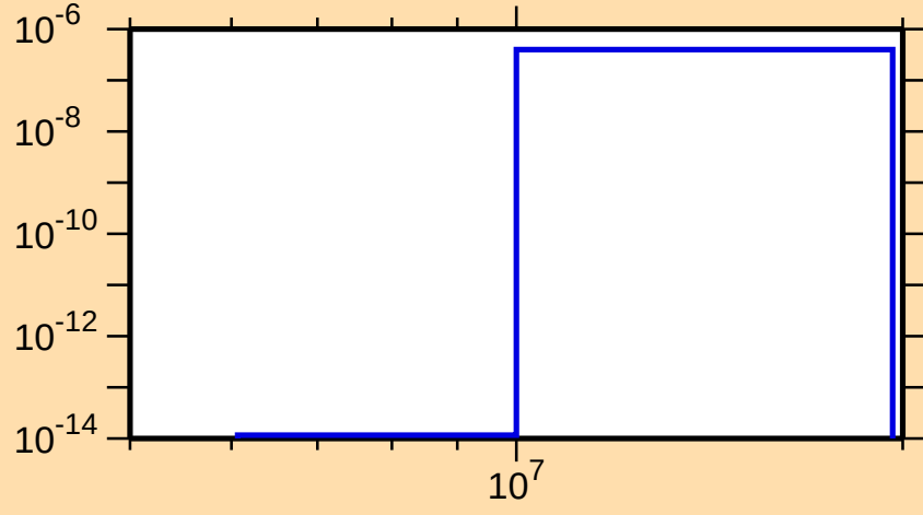
\sigma vs. E for ^{117}\text{Xe}(\text{mt117})
