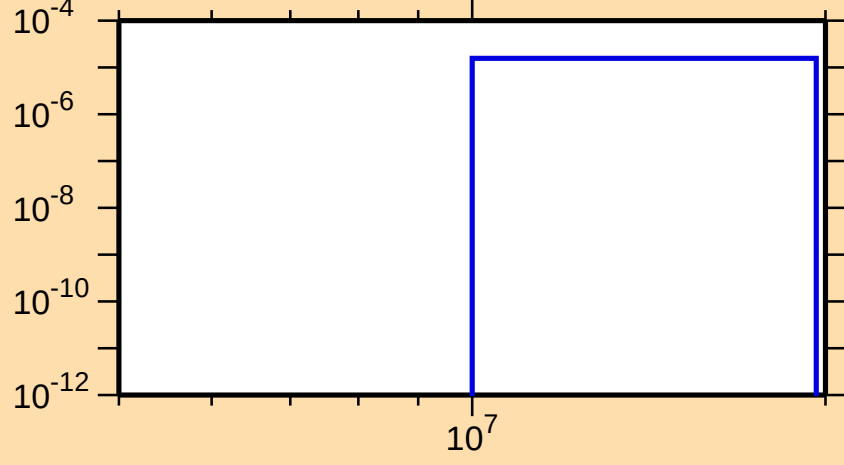
\sigma vs. E for ^{117}\text{Xe}(\text{mt } 45)
