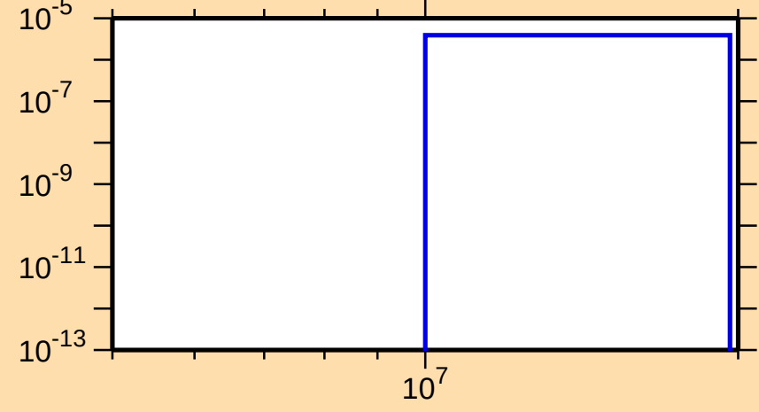
\sigma vs. E for ^{117}\text{Xe}(n,\text{pt})
