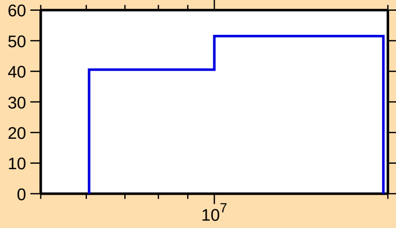
\Delta\sigma/\sigma vs. E for ^{117}\text{Xe}(n,\text{inel.})
