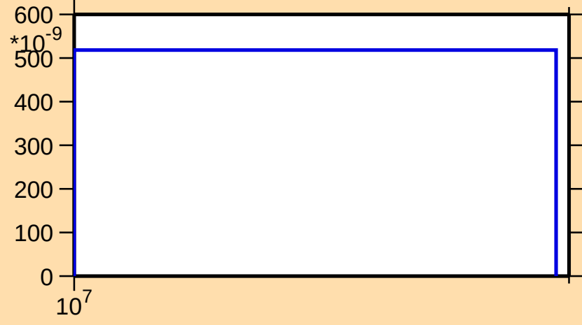
\sigma vs. E for ^{117}\text{Xe}(n,\text{nd})
