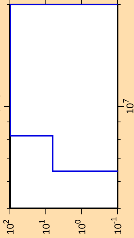
\Delta\sigma/\sigma vs. E for ^{117}\text{Xe}(n,t)
