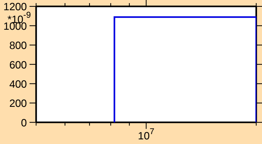
\sigma vs. E for ^{117}\text{Xe}(n,2n\alpha)
