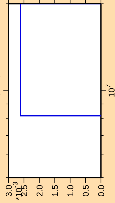
\Delta\sigma/\sigma vs. E for ^{117}\text{Xe}(n,nt)
