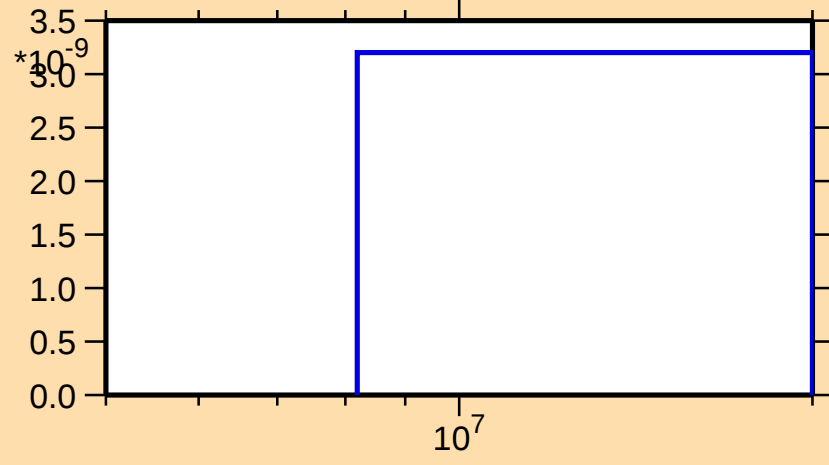
\sigma vs. E for ^{117}\text{Xe}(\text{mt } 34)
