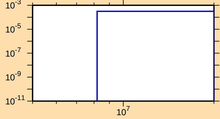
\sigma vs. E for ^{117}\text{Xe}(n,t)
