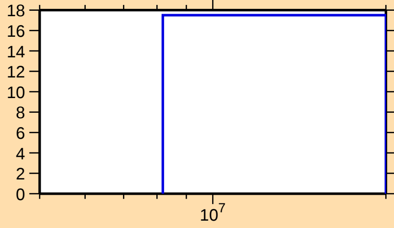
\Delta\sigma/\sigma vs. E for ^{117}\text{Xe}(n,\text{nonel.})
