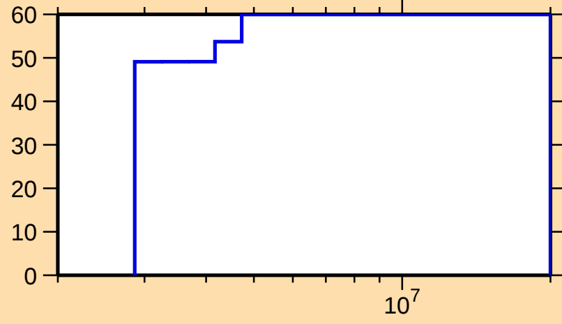
\Delta\sigma/\sigma vs. E for ^{118}\text{Xe}(n,n_1)
