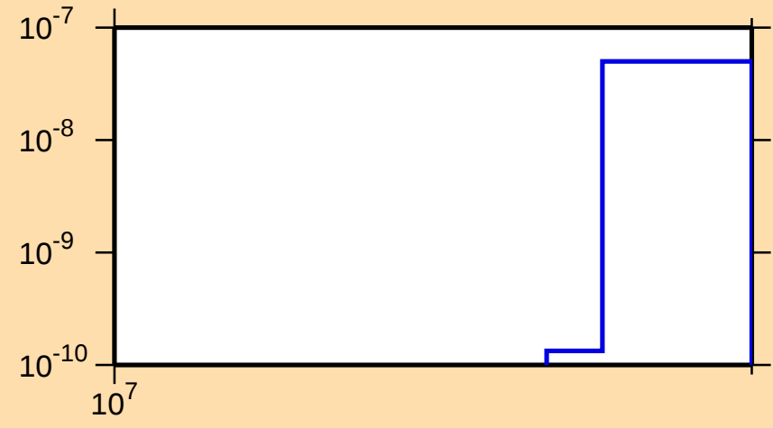
\sigma vs. E for ^{118}\text{Xe}(n,\text{pt})
