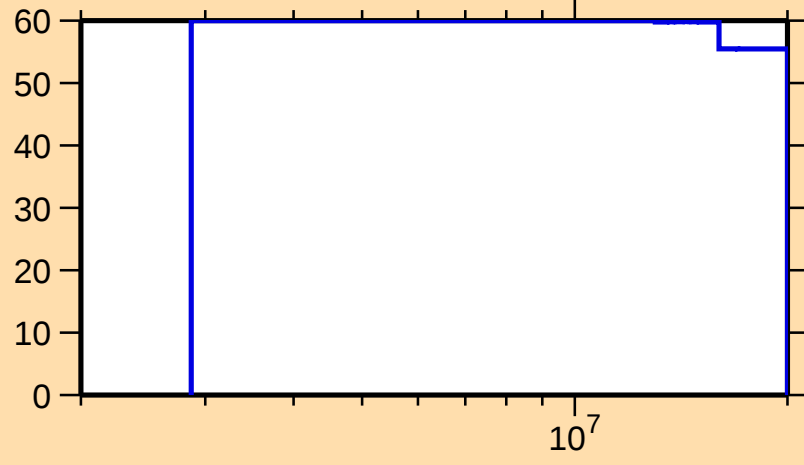
\Delta\sigma/\sigma vs. E for ^{118}\text{Xe}(n,n\text{cont.})
