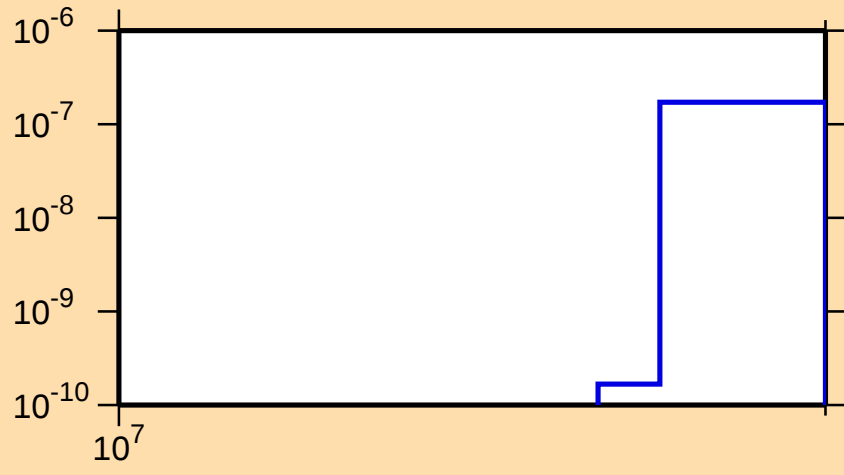
\sigma vs. E for ^{118}\text{Xe}(n,\text{nd})
