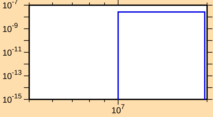
\sigma vs. E for ^{118}\text{Xe}(\text{mt117})
