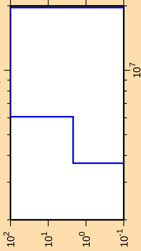
\Delta\sigma/\sigma vs. E for ^{118}\text{Xe}(n,\text{He3})
