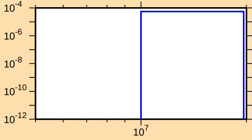
\sigma vs. E for ^{118}\text{Xe}(n,t)
