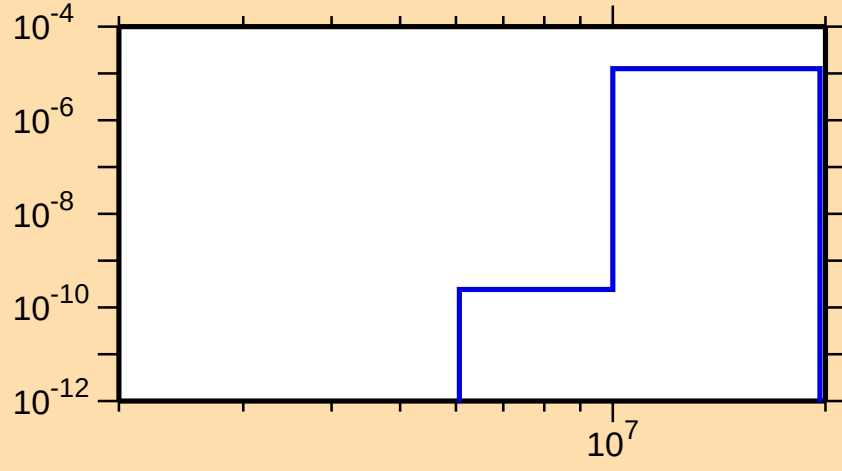
\sigma vs. E for ^{118}\text{Xe}(n,\text{He3})
