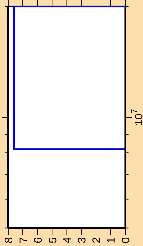
\Delta\sigma/\sigma vs. E for ^{118}\text{Xe}(\text{mt } 34)
