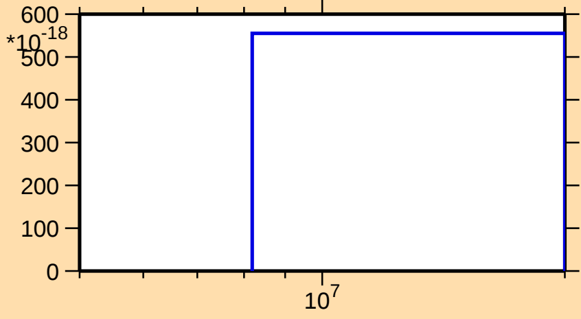
\sigma vs. E for ^{118}\text{Xe}(n,nt)
