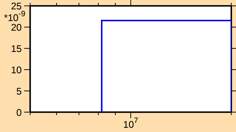
\sigma vs. E for ^{118}\text{Xe}(\text{mt117})
