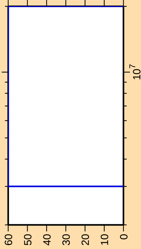
\Delta\sigma/\sigma vs. E for ^{118}\text{Xe}(n,\text{ncont.})
