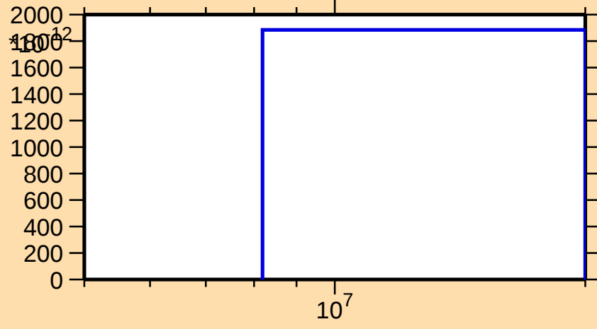
\sigma vs. E for ^{118}\text{Xe}(n,2n\alpha)
