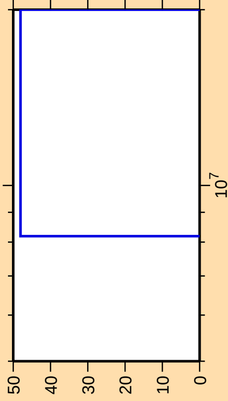
\Delta\sigma/\sigma vs. E for ^{118}\text{Xe}(\text{mt } 45)
