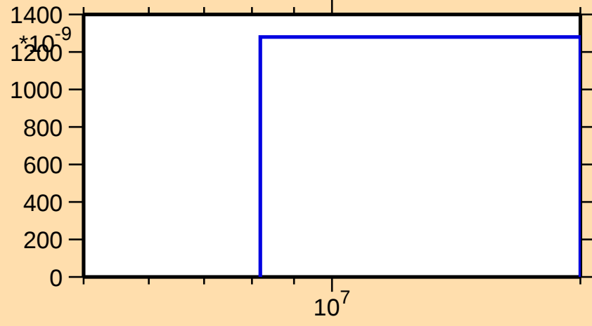
\sigma vs. E for ^{118}\text{Xe}(\text{mt } 45)
