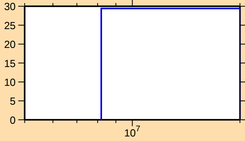
\Delta\sigma/\sigma vs. E for ^{118}\text{Xe}(n,\text{inel.})
