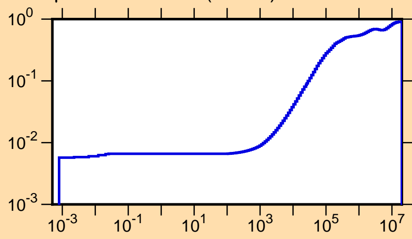
\mu vs. E for ^{119}\text{Xe}(\text{mt251})
