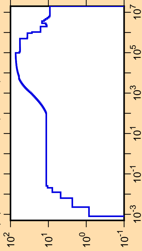
\Delta\mu/\mu vs. E for ^{119}\text{Xe}(\text{mt251})
