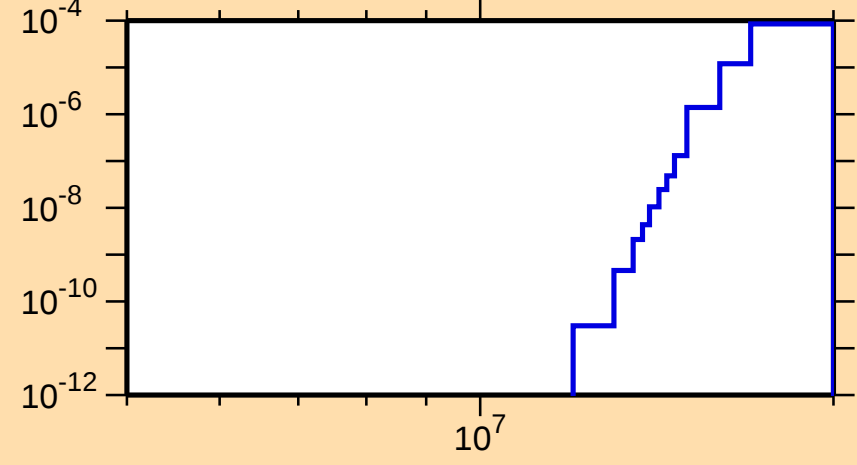
\sigma vs. E for ^{119}\text{Xe}(n,2n\alpha)
