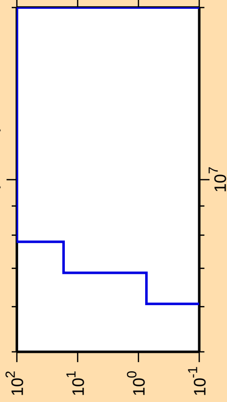
\Delta\sigma/\sigma vs. E for ^{119}\text{Xe}(n,\text{He3})
