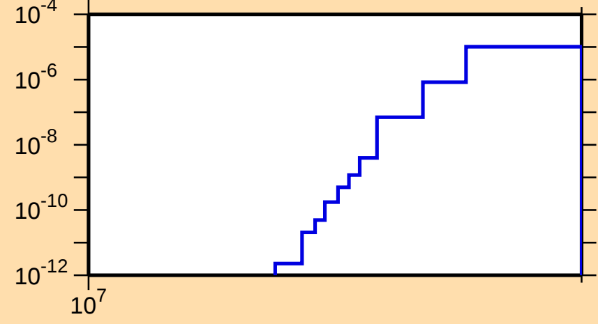
\sigma vs. E for ^{119}\text{Xe}(n,\text{pt})
