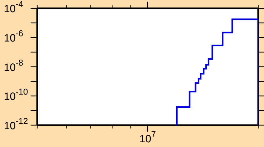
\sigma vs. E for ^{119}\text{Xe}(\text{mt } 45)
