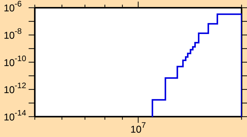
\sigma vs. E for ^{119}\text{Xe}(\text{mt117})
