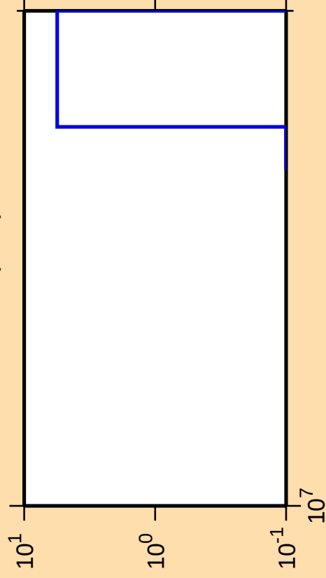
\Delta\sigma/\sigma vs. E for ^{119}\text{Xe}(n,nt)
