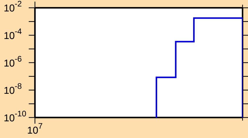
\sigma vs. E for ^{119}\text{Xe}(n,2np)
