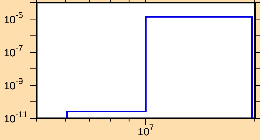
\sigma vs. E for ^{119}\text{Xe}(n,\text{He3})
