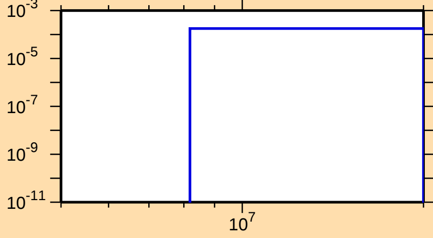
\sigma vs. E for ^{119}\text{Xe}(n,t)
