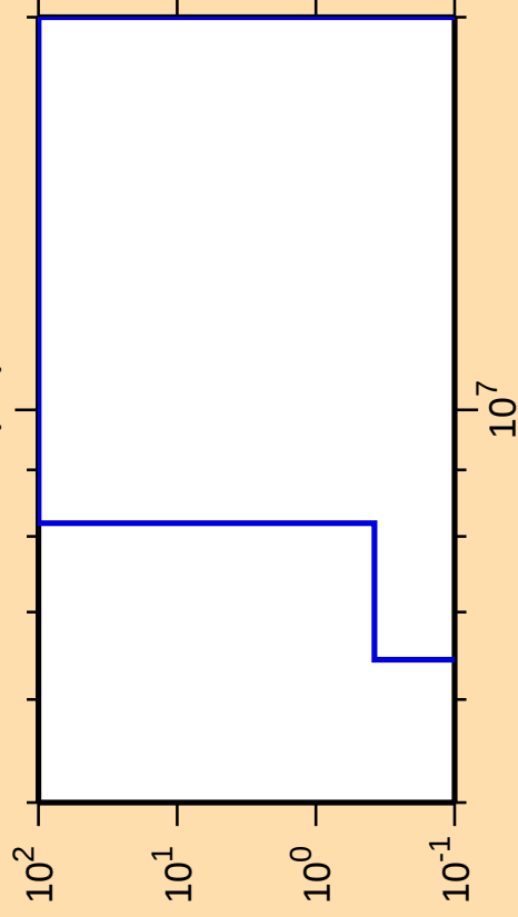
\Delta\sigma/\sigma vs. E for ^{119}\text{Xe}(n,t)
