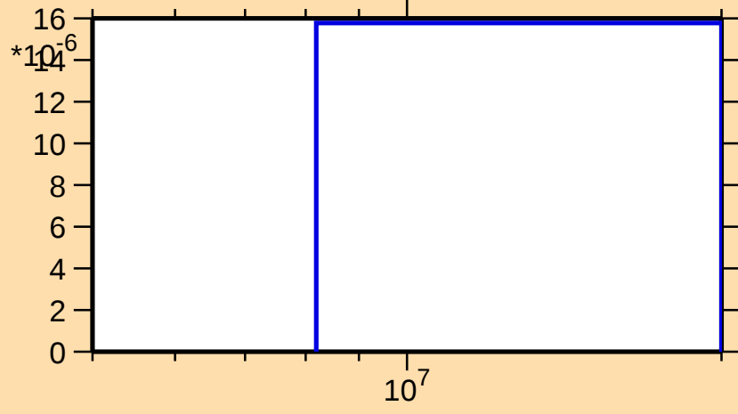
\sigma vs. E for ^{119}\text{Xe}(n,2np)
