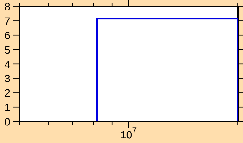
\Delta\sigma/\sigma vs. E for ^{119}\text{Xe}(n,\text{tot.})
