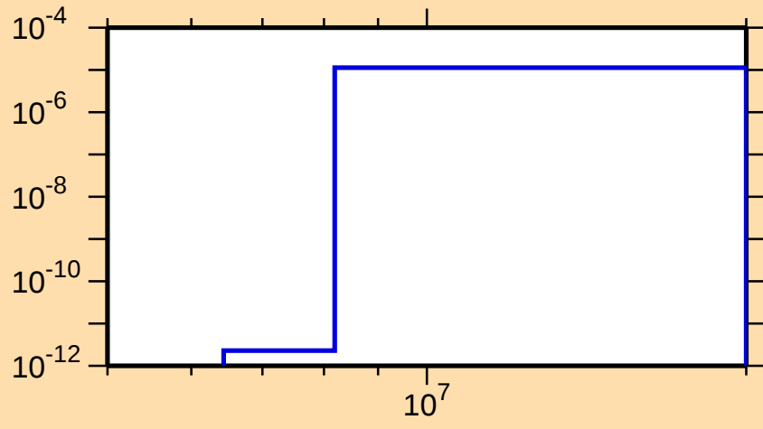
\sigma vs. E for ^{119}\text{Xe}(n,\text{He}3)
